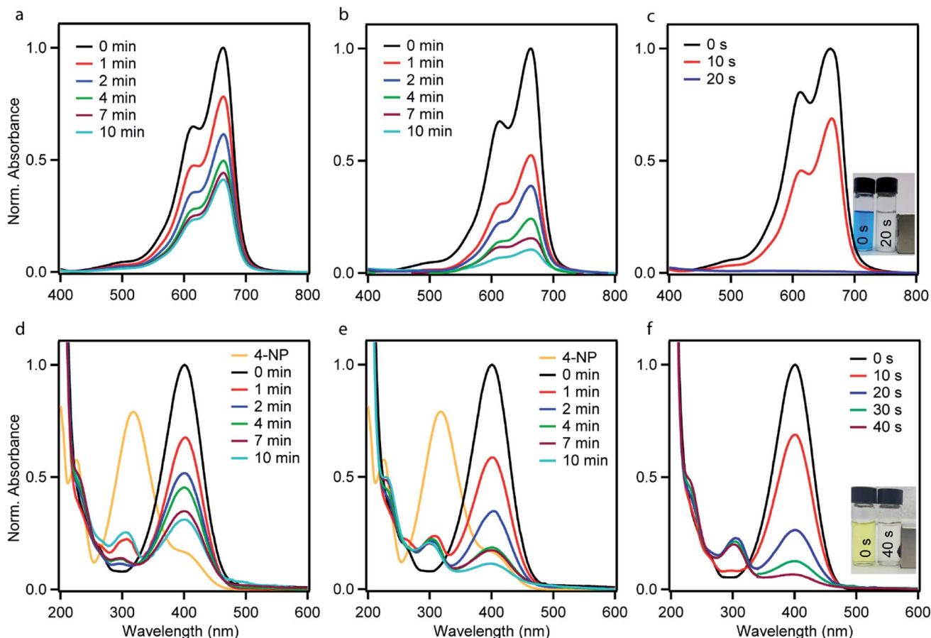
Fig. 4 The representative UV-vis absorption spectra of an aqueous MB solution in the presence of NaBH 4 using (a) Ni-PD (b) PD-Au (c) Ni-PD-Au as catalysts, and UV-vis absorption spectra of an aqueous 4-NP solution in the presence of NaBH 4 using (d) Ni-PD (e) PD-Au (f) Ni-PD-Au as catalysts monitored as a function of time.
