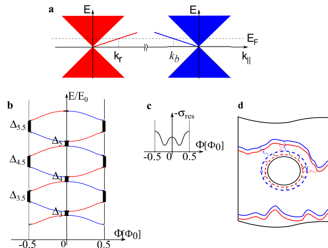
Figure 4 | Edge states around the graphene nanohole. (a) The red and blue rays are the Tamm-Dirac states contra-propagating along the graphene semi-plane. There are two Tamm-Dirac states at the Fermi level: k_r in the red valley with positive velocity and k_b in the blue valley with negative velocity. The bulk continuum states are shadowed. (b) Spectrum of the Tamm-Dirac states in an antidot for different j_+, j_- as a function of the magnetic flux that passes through the antidot area. The spectrum has a band character, and the flow through the antidot plays a role of quasi-momentum in the reduced zone scheme. The red (blue) colour corresponds to the valley with \tau = +1 ( \tau = -1 ), E_0 \approx 2a\hbar v/R . The red-blue scattering results in band gaps (vertical bold lines). Gaps are formed by anticrossing of red and blue edge states with angular momenta j_+ and j_- . Gap values are denoted by the index j = (j_+ + j_-)/2 . (c) Inter-valley contribution to the conductivity in the reduced zone scheme. The peaks correspond to resonant red-blue back-scattering. The two series of peaks are connected by the passing of the magnetic flux through the centre and boundary of the zone shown in panel (b). (d) Contra-propagating trajectories of the orbit centres for different valleys for the zero Landau level ( N=0 ) in a smooth-impurity potential. One of the orbits is close to the antidot and can experience inter-valley back-scattering at the above-mentioned values of the flux.
