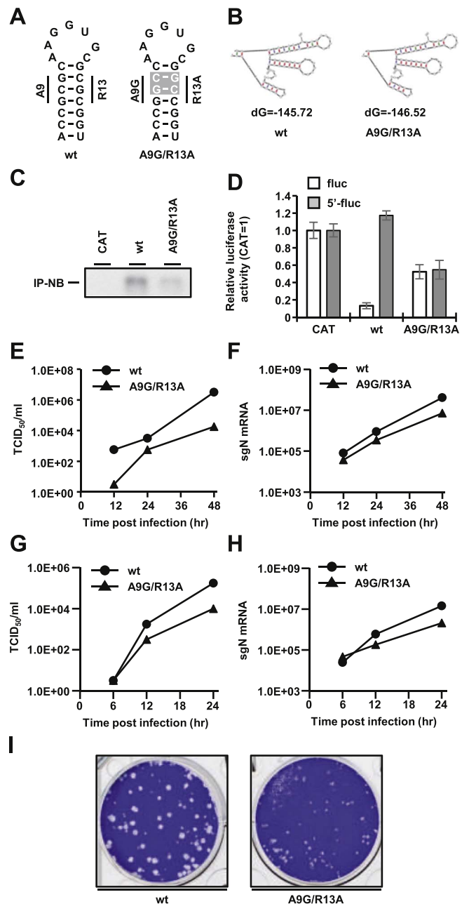
Fig. 6. Rigorous viral RNA recognition by nsp1 in viral replication. (A) The predicted SL5C in MERS-CoV structures of the wt (left) and A9G/R13A mutant (right). Introduced nucleotide mutations are shown in a gray box with white letters. (B) Partial RNA structures of the wt (left) and A9G/R13A mutant (right) of MERS-CoV from the region in the black square in Fig. 5D. Free energies (dG) are shown below. (C) Lysates of 293T cells transfected with either pCAG-CAT, pCAG-nsp1 or pCAG-nsp1-A9G/R13A together with pCAG-5'-fluc were immunoprecipitated with anti-FLAG antibody at 24 h posttransfection. RNAs extracted from the precipitates were subjected to Northern blot analysis using a riboprobe for the luciferase gene. (D) Luciferase activities in 293T cells transfected with either pCAG-fluc or pCAG-5'-fluc together with the indicated expression plasmids were determined at 24 h posttransfection after standardization with those in cells expressing CAT. The values represent the means \pm SD from three independent experiments. (E, F) Vero cells were infected with each recombinant MERS-CoV at an MOI of 0.001, and the virus titers of culture supernatants (E) and levels of subgenomic N mRNA in infected cells (F) were determined at 12, 24 and 48 h postinfection. Because the values of mock samples were under LOD, the data of mock were not shown. (G, H) Huh7 cells were infected with each recombinant MERS-CoV at an MOI of 0.001, and the virus titers of culture supernatants (G) and levels of subgenomic N mRNA in infected cells (H) were determined at 6, 12 and 24 h postinfection. Because the values of mock samples were under LOD, the data of mock were not shown. (I) Plaque morphology of the wt and nsp1-A9G/R13A mutant MERS-CoVs following agarose overlay plaque assay using Vero cell. Infected cells were fixed with phosphate-buffered formaldehyde at 3 days postinfection and stained using crystal violet.
