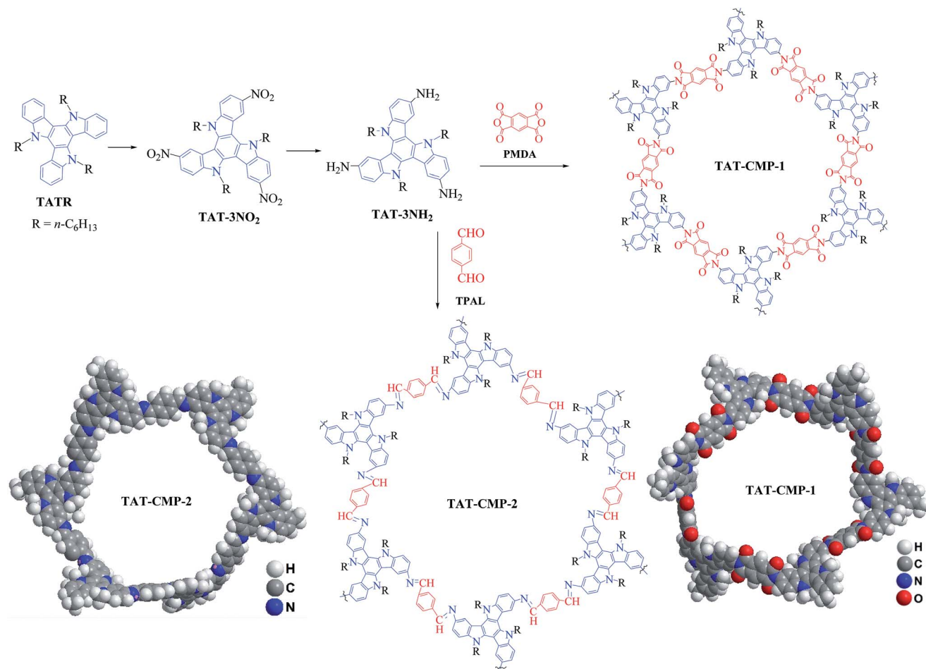
Fig. 1 Synthesis route and the three-dimensional view of TAT-CMP-1 and TAT-CMP-2 in an amorphous periodic cell (grey: carbon, white: hydrogen, blue: nitrogen, red: oxygen, and n -hexyl groups ( R ) are omitted for clarity).
