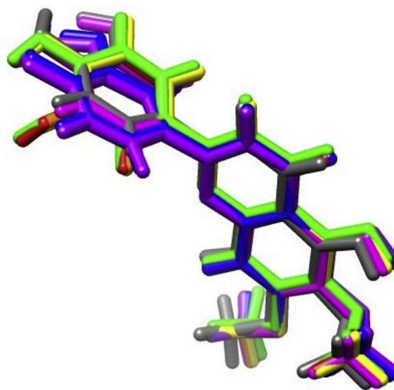
Fig. 4. The eight best conformations of CIR after molecular docking in CD.
