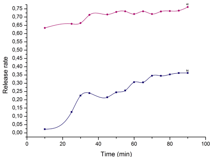
Fig. 6. In vitro release study of CD-CIR inclusion complex (a) and CIR (b) in an acidified saline solution (pH 1.5).
