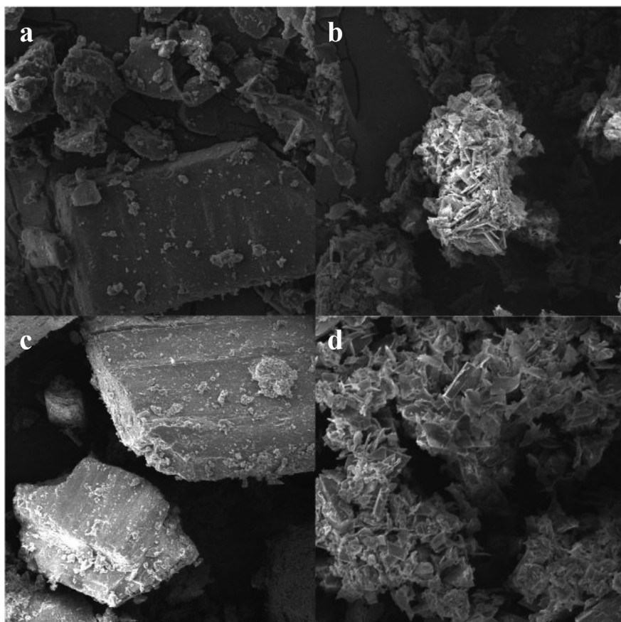
Fig. 1. SEM micrographs: a) beta-cyclodextrin (CD); b) cirsiolol (CIR); c) PM-CD-CIR; d) CD-CIR. PM = physical mixture. VEGAN3 TESCAN images with increase 2 K (bar = 20 \mu\text{m} ).
