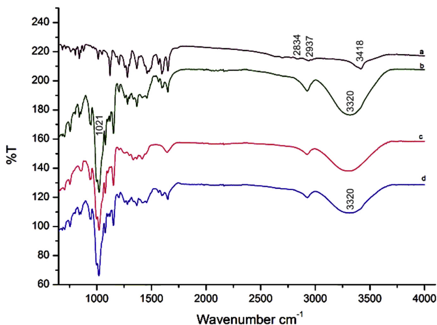
Fig. 2. FTIR spectra a) cirsioliol; b) inclusion complex CD-CIR; c) CD; d) PM-CD-CIR; PM = physical mixture.
