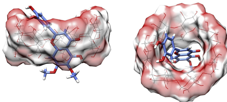
Fig. 5. Best docking conformation for CIR-CD in two visualization modes (the surfaces denote the occupation volume of CD based on Van der Waals radii). CD = \beta -cyclodextrin; CD-CIR = inclusion complex (1:1) \beta -cyclodextrin-cirsiliol.
