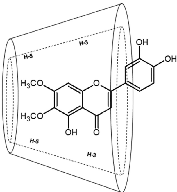
Fig. 3. Possible inclusion mode of cirsiliol in cavity of \beta -cyclodextrin.
