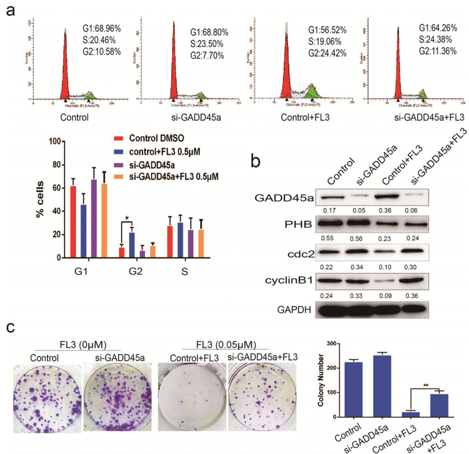
Fig. 4 Repression of GADD45a decreases the inhibitory effect of FL3 on cell cycle progression. a Flow cytometry assay was performed in T24 cells to measure the effect of FL3 on the cell cycle distribution in the presence or absence of siGADD45a-RNA. The percentage of cells in each phase was shown in the histograms; data represent the mean \pm SD of three independent experiments, * P < 0.05 indicates a significant difference. b Total cell lysates from indicated T24 cells (up panel) were harvested and subjected to Western blot analysis with the indicated proteins (left panel). c Cell colony formation experiments were performed to measure the inhibitory effect of FL3 on cell proliferation of T24 cells in the presence or absence of GADD45a. Histograms represent the mean \pm SD numbers of colonies of three independent experiments. ** P < 0.01 indicates significance
