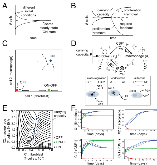
Fig. 1. Homeostasis of cell numbers through circuits of communicating cells. (A) An ON state exists when cell numbers converge to the same steady-state concentration starting from a range of different initial conditions. (B) The ON state requires careful regulation, because if proliferation and removal rates are unequal cells rise to a high carrying capacity or decline to zero. (C) A schematic phase portrait of the FB–MP coculture experiment, showing its three fixed points: a stable OFF state (red), a stable ON state (blue), and an ON–OFF state (green). (D) The FB–MP circuit topology: CSF1 cross-inhibits PDGF gene expression, FB and MP endocytose their GFs, and FB secrete PDGF. (Lower) Description of the interactions in the circuits. (E) The phase portrait of the FB–MP circuit provided by the model of Eqs. 1–4, using the biologically plausible parameter values \lambda_1 = 3.7 , \lambda_2 = 2.2 , \mu = 1 , \beta_{12} = 3.4 , \beta_{11} = 6.8 , and \alpha_{12} = 10 , \alpha_{21} = 1 . The axes are dimensionless cell numbers, with conversion factors to cell numbers shown. Examples of trajectories that go to each fixed point are shown in color. (F) Dynamics of the cell and GF concentrations for the trajectories highlighted in E as well as two other trajectories for each fixed point.
