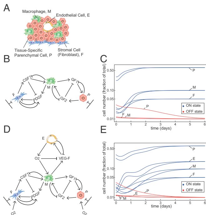
Fig. 4. The two-cell circuits can scale up to form a modular, bistable circuit made of three and four cell types. (A) A typical tissue unit made of parenchymal cells, macrophages, fibroblasts, and endothelial cells. (B) A three-cell circuit topology made of modules of the observed two-cell circuit topology. Fibroblasts (F) and parenchymal cells (P) have a carrying capacity, whereas macrophages (M) are far from carrying capacity. In this circuit, macrophages integrate the responses of the other two cell types. (C) Dynamics of cell numbers show that all cell types converge to an ON steady state from a wide range of initial conditions (blue curves). For initial cell numbers below a threshold cells decline to zero (OFF state, red lines). The parameters used are \beta_{12} = \beta_{23} = \beta_{32} = 10 , \beta_{11} = 5 , \alpha_{12} = \alpha_{21} = \alpha_{23} = \alpha_{32} = 10 , and \lambda_1 = \lambda_2 = \lambda_3 = 10 . (D) A four-cell circuit topology made of modules of the observed two-cell circuit topology with endothelial cells (E) that are far from carrying capacity. (E) The same as in C with the parameters \beta_{12} = \beta_{23} = \beta_{32} = \beta_{24} = \beta_{42} = 10 , \beta_{11} = 5 , \alpha_{12} = \alpha_{21} = \alpha_{23} = \alpha_{32} = \alpha_{24} = \alpha_{42} = 10 , and \lambda_1 = \lambda_2 = \lambda_3 = \lambda_4 = 10 .
