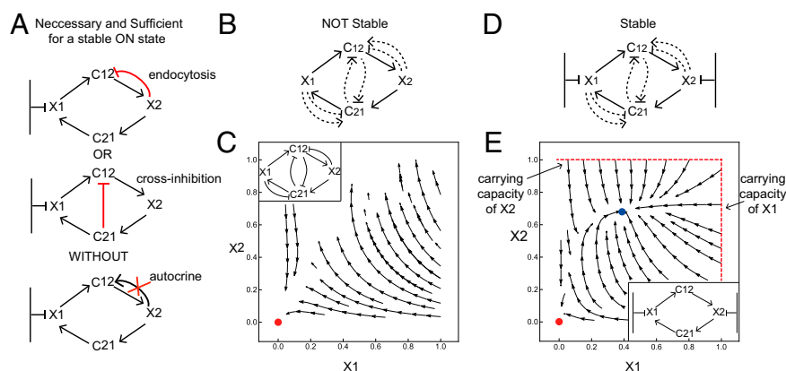
Fig. 2. A necessary and sufficient condition for a stable ON state in cell circuits. (A) The GF for the cell that is far from carrying capacity ( C_{12} ) must be inhibited either by endocytosis or by cross-regulation and must have no autocrine loop. (B) Circuits in which neither cell type is close to carrying capacity do not have a stable ON state. (C) Stream plot of one of the circuits in B shows that cell numbers either degenerate to zero (marked in red) or grow without bound. (D) Circuits in which both cells are close to carrying capacity are stable with no need for cross-regulation or feedback. (E) Stream plot of one of the circuits in D shows that even without regulation on the GFs cells reach either an OFF state (marked in red) or an ON state (marked in blue).
