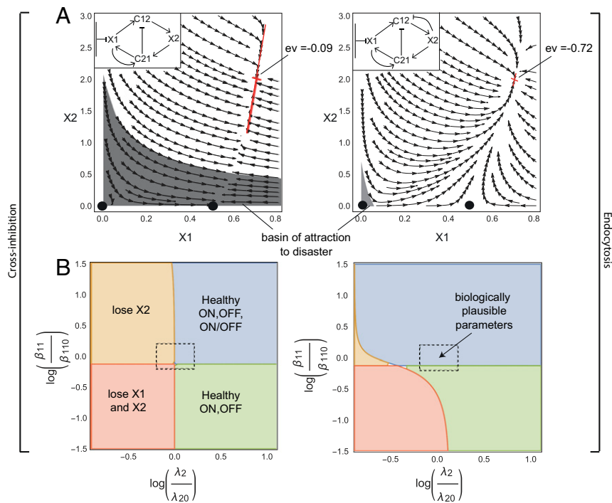
Fig. 3. Endocytosis is a more robust and rapid mechanism than cross-regulation for cell circuits to stabilize their ON state. (A) A mathematically controlled comparison of endocytosis and cross-inhibition mechanisms shows that endocytosis (Right) provides a smaller basin of attraction for losing one or both cell types (gray region). The endocytosis circuit also reaches the stable ON state eightfold faster, as indicated by its more negative Jacobian eigenvalue (ev) at the fixed point. (B) The circuit with endocytosis is more robust with respect to parameter variation than the circuit with cross-inhibition, in the sense that it is less prone to lose one or both cell types. The center of the dashed rectangle corresponds to parameter values of \bar{\lambda}_1=8 , \bar{\lambda}_2=8 , \bar{\mu}=1 , \bar{\beta}_{11}=4.4 , and \bar{\alpha}_{21}=15.0 . For the circuit with cross-inhibition (Left) \bar{\beta}_{12}=0.35 and \bar{\alpha}_{12}=0.001 . For the circuit with endocytosis (Right) \bar{\beta}_{12}=1.99 and \bar{\alpha}_{12}=5 . Axes are log relative variation from these parameters.
