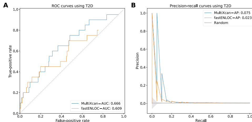
Fig. 3. PhenomeXcan validation using a curated list of causal genes in type 2 diabetes. MultiXcan refers to the version of PrediXcan designed to take GWAS summary statistics and aggregate results across tissues (22). (A and B) ROC and PR curve of PrediXcan significance scores (blue) and fastENLOC (orange) to predict significant associations between a curated gene list from the AMP T2D Knowledge Portal and type 2 diabetes traits. PrediXcan and fastENLOC, particularly PrediXcan, demonstrate predictive ability in the setting of a disease trait with 20 genes with causal, strong, and moderate evidence and present in LD blocks with GWAS signal. The maximum fastENLOC colocalization probability across tissues was used for all figures.
