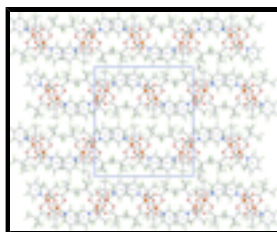
Fig. 3. Packing of layers in (I) along the b axis. Colour code: Cu, orange; O, red; N, blue; C, grey; and H, green.
