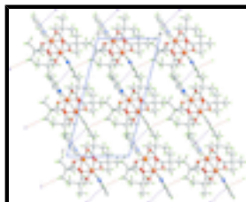
Fig. 2. The 2-D array in the ac plane in (I) mediated by \pi - \pi and C—H \cdots \pi interactions, shown as purple and orange dashed lines, respectively. Colour code: Cu, orange; O, red; N, blue; C, grey; and H, green.
