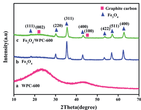
Fig. 1 XRD patterns of (a) WPC-600, (b) pure Fe 3 O 4 and (c) Fe 3 O 4 /WPC-600 composite.
