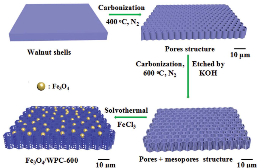
Scheme 1 Demonstration of fabrication process used for Fe 3 O 4 /WPC-600 composite materials.
