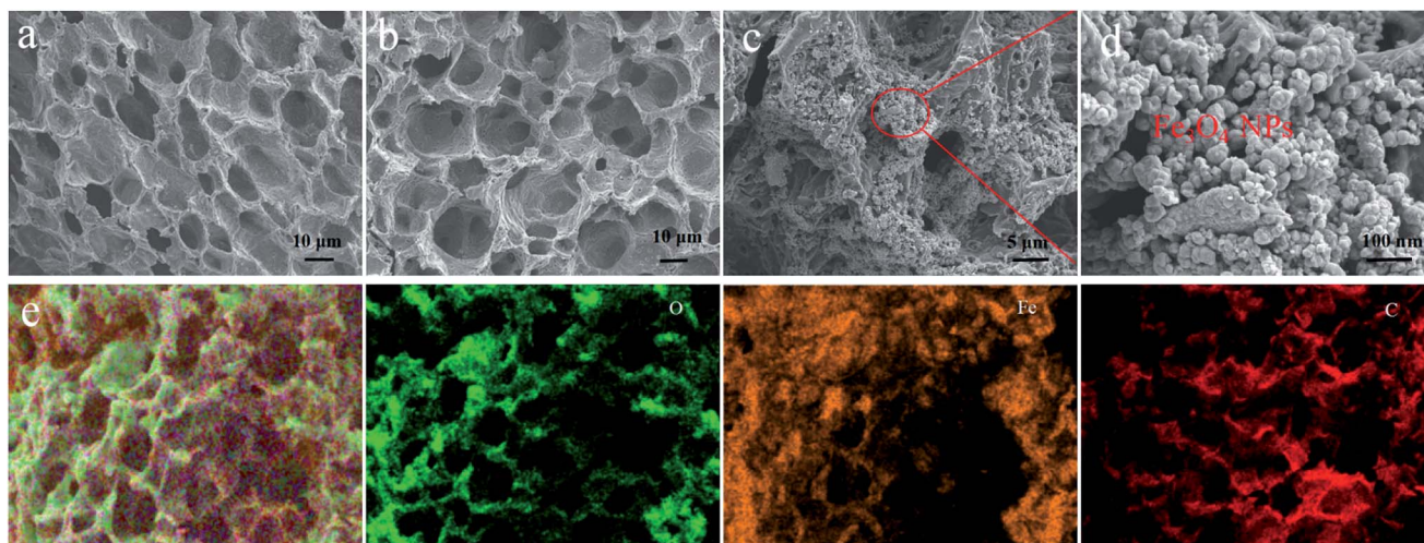
Fig. 2 SEM images of WC-600 (a), WPC-600 (b) and Fe 3 O 4 /WPC-600 at different magnifications (c and d); EDS elemental mapping images of Fe 3 O 4 /WPC-600 (e).
