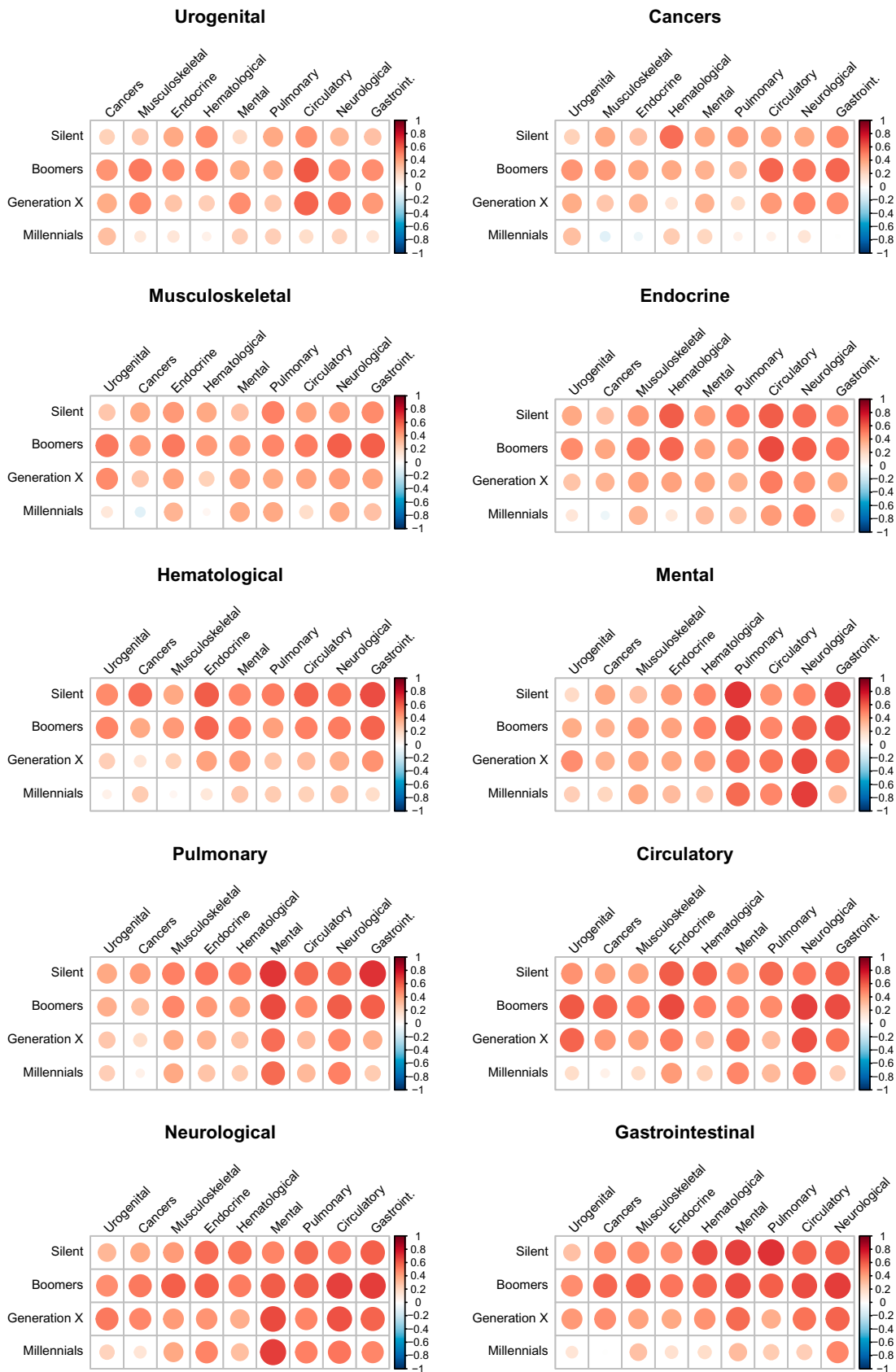
Fig. 4. Genetic correlations of each of 10 broad diagnostic categories with the remaining nine by demographic cohort. Only the four most data-rich cohorts—Silent Generation, Baby Boomers, Generation X, and Millennials—were considered. Estimates were based on averages from all available relative pairs within a radius of three meioses weighted by sampling variance. Blank cells correspond to correlations not significantly different from zero.
