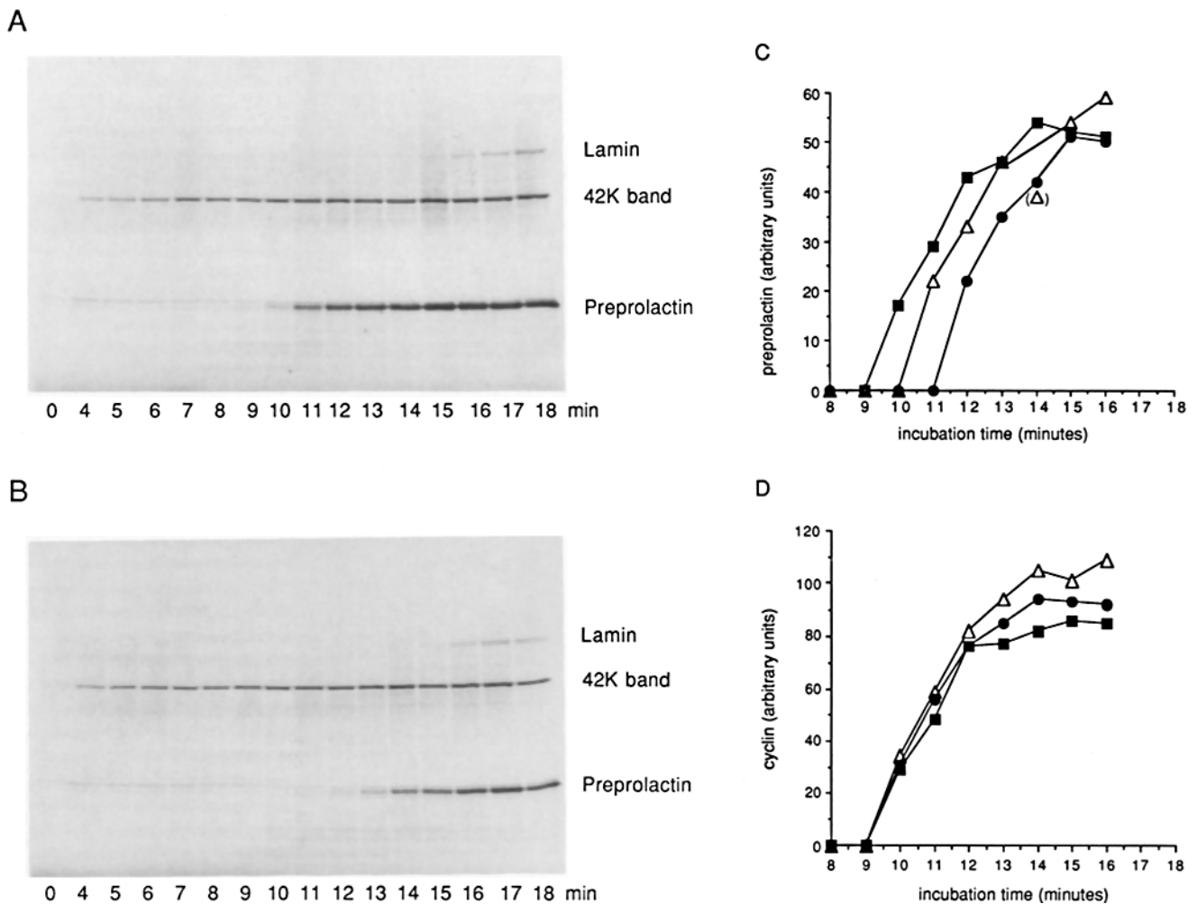
Figure 1. Addition of canine SRP delays synthesis of preprolactin in reticulocyte lysates. (A and B) Synthetic mRNAs encoding either bovine preprolactin or Xenopus lamin L 1 were translated in a synchronized rabbit reticulocyte lysate as described in Materials and Methods. The translation reaction contained either (A) no added canine SRP or (B) 200 nM SRP. Aliquots were sampled at the times shown and analyzed by SDS-PAGE. The band labeled 42K is due to posttranslational addition of methionine to an endogenous lysate protein (Jackson and Hunt, 1983). (C and D) Synthetic mRNAs encoding either bovine preprolactin (C) or sea urchin cyclin (D) were translated in a synchronized rabbit reticulocyte lysate as described in Materials and Methods. Translation reactions contained either no added SRP (■), 30 nM SRP (●), or 100 nM SRP (Δ). Aliquots were sampled at the times indicated and analyzed by SDS-PAGE and scanning densitometry as described.
