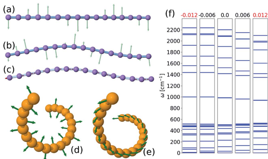
Fig. 4 Phonon normal modes of a two-dimensional 16-atom chain under -0.015 strain and three-dimensional 20-atom chain under 0.04 strain: (a) 10 th mode with a frequency of 95 cm -1 ; (b) 13 th mode with a frequency of 212 cm -1 ; (c) 41 st mode with a frequency of 1728 cm -1 ; (d) mode number 34; (e) mode number 4. (a)–(c) are two dimensional, and (d) and (e) are three dimensional; (a) is rotated 90° about the chain axis, and the vibrations are normal to the bending plane; the arrow lengths are the scaled displacements of each mode, and (f) T point phonon frequencies of a chain with a 16-atom unit cell.
