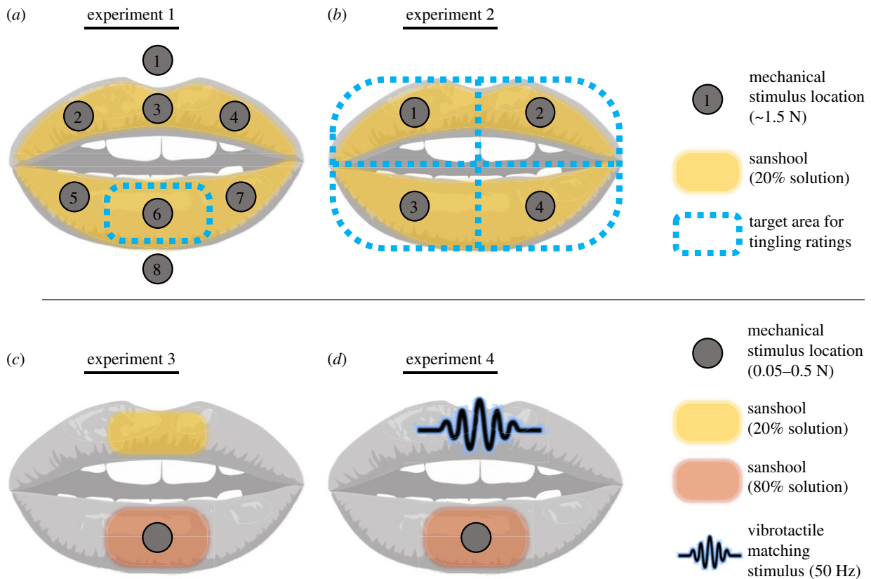
Figure 1. Experimental methods. (a,b) In experiments 1 and 2, participants experienced sanshool tingling all over the lips, while sustained touch (approx. 1.5 N) was manually applied in different locations for 10 s. Participants reported the effect of touch location on sanshool tingling by rating the change in tingling intensity on the centre of the lower lip (a: experiment 1) or all over the lips (b: experiment 2). (c) In experiment 3, weaker and stronger sanshool solutions caused weaker and stronger tingling intensities on the upper and lower lips, respectively. Different levels of sustained force (0.05, 0.1625, 0.275, 0.375 and 0.5 N) were then applied to the lower lip by a closed-loop robotic device (electronic supplementary material, figure S2). Participants reported which lip had the strongest tingling, as a function of sustained force. (d) In experiment 4, participants estimated the intensity of sanshool tingling on the lower lip by adjusting the amplitude of 50 Hz vibration applied to the upper lip until the intensities felt equal. Meanwhile, different levels of sustained force (0.05, 0.20 or 0.35 N) were applied on the lower lip. The adjustment was done at four different timings from the onset of the force (before pressure, and at 0, 5 and 10 s after pressure) (electronic supplementary material, video). (Online version in colour.)
