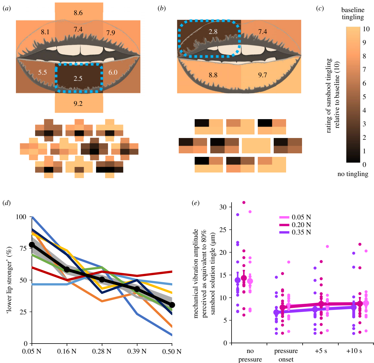
Figure 2. Results. ( a–c ) Mean (top) and individual (bottom; n = 10 in each experiment) perceived intensity of sanshool tingling as a function of touch location in experiments 1 ( a ) and 2 ( b ). Colour indicates the perceived intensity relative to the baseline period ( c ) (darker colours indicate lower ratings). In experiment 1 ( a ), the perceived intensity of sanshool tingling at the target location (centre of lower lip) dropped significantly when sites on the lower lip were touched by the probe. In experiment 2 ( b ), touch was applied to each of four quadrants in random order. Each time touch was applied, participants gave separate tingling ratings for each quadrant, after being prompted in random order. Data from all four touch conditions were realigned to the left upper lip position to express the spatial relation between the location where tingling intensity was judged and the location where sustained touch was applied. Significant intensity reduction was observed at the location where the touch was applied. ( d ) In experiment 3 ( n = 8 ), the probability of judging the lower lip tingling intensity as stronger than the upper lip decreased as force level increased. The black line represents the sample average, the grey shading represents the s.e.m., and coloured lines represent individual data. ( e ) In experiment 4 ( n = 14 ), the estimated vibration amplitude of sanshool tingling decreased as a static force increased. Moreover, the intensity of tingling significantly recovered as time elapsed. Error bars indicate the s.e.m. across participants and coloured dots indicate individual data. (Online version in colour.)
