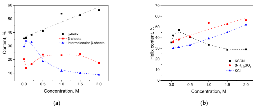
Figure 18. Changes in the secondary structure of HSA in the interaction with (\text{NH}_4)_2\text{SO}_4 (a) and salt-specific effects on the \alpha -helical secondary structure of HSA(b) in 10% wt. aqueous solution at 80 °C.
