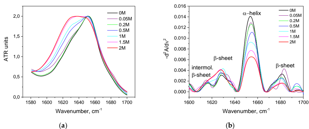
Figure 2. Changes in the Amide I band (a) and changes in the second derivative of the Amide I band (b) of HSA in 10% wt. aqueous solution at 23 °C with various concentrations of KSCN.
