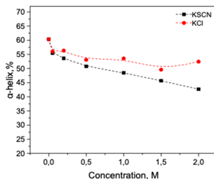
Figure 7. Salt-specific effects on the \alpha -helical secondary structure of HSA measured by the FTIR spectroscopy.
