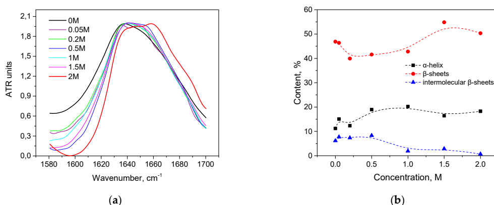
Figure 10. Changes in the character of the Amide I band (a) of trypsin at 23 °C with various concentrations of (NH 4 ) 2 SO 4 and ammonium sulfate-induced conformational transition of trypsin at 23 °C (b). Protein concentration was 20% wt.
