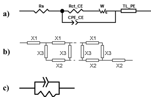
Fig. 15 (a) Equivalent circuit used to adjust the impedance spectra of the manufactured DSSCs. The transmission line TL_{PE} follows the scheme shown in (b), where each element X_1 , X_2 and X_3 becomes a resistor and a phase element in parallel, as shown in (c).
