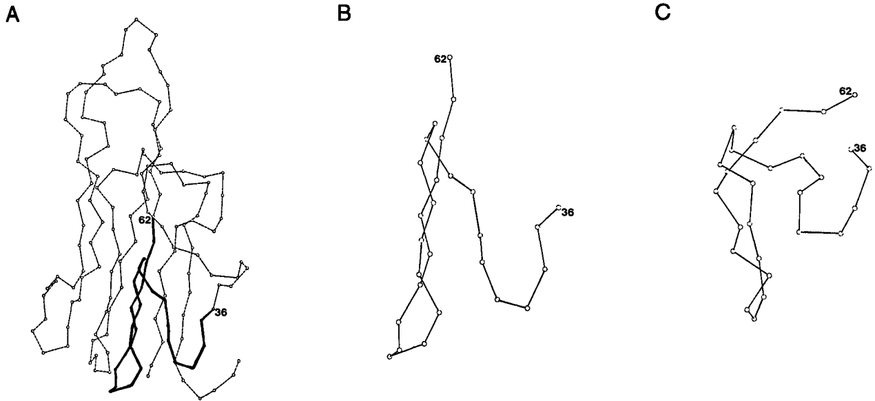
FIG. 1. Drawing of the TNF \alpha monomer and the TNF \alpha 36-62 peptide. (A) Drawing of the \alpha -carbon backbone of the minimized crystal structure of TNF \alpha . The sequence consisting of residues 36-62 are blackened. (B) Drawing of the \alpha -carbon backbone of the TNF \alpha sequence 36-62. (C) Drawing of the minimized structure of the TNF \alpha 36-62 \alpha -carbon backbone based on molecular modelling, using Computer Graphics.
