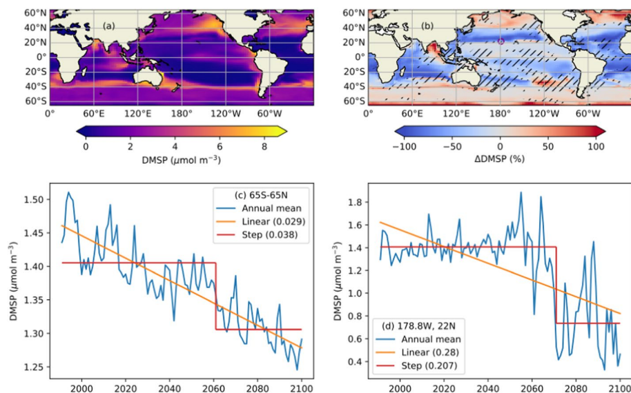
Fig. 6 Abrupt shifts in dimethylsulfoniopropionate (DMSP) in the global ocean during the twenty-first century derived from the output of a 35-compartment phytoplankton model projection based on a high greenhouse gas emission scenario. a Global distribution of annual mean sea surface DMSP averaged over 2005–2024, b projected percentage change in annual mean sea surface DMSP averaged over 2081–2100 relative to the period 2005–2024, and time series of annual mean sea surface DMSP c averaged over 65°S–65°N and d at a location in the North Pacific subtropical gyre denoted by a purple circle in b . DMSP is derived by multiplying the modelled carbon biomass of dinoflagellates by 22, coccolithophores by 11, diatoms by 0.86, and diazotrophs/prokaryotes/picocaryotes by 0.0015, which are the observed mean intracellular ratios for these phytoplankton functional types (Stefels et al. 2007; M. Galí and J. Stefels, personal communication, September 2023). In b , hatches represent areas where the step-function outperforms the linear regression in fitting the projected time series over 1991–2100 at each grid point. In c and d , orange and red lines represent the best fit based on linear regression and step function, respectively. Numbers in parentheses represent the root mean square error of each fit. See the main text for details
