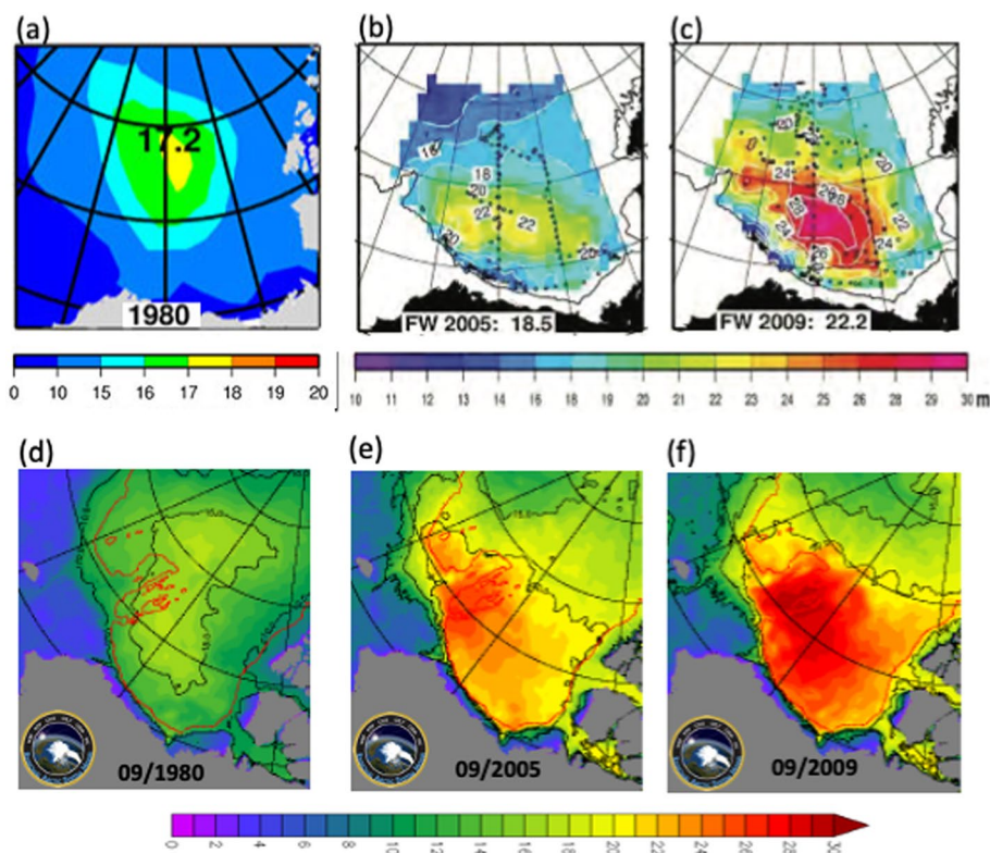
Fig. 3 Estimates of the BG freshwater content (in meters) from observations (top; https://www2.whoi.edu/site/beaufortgyre/ ) and the high-resolution Regional Arctic System Model (RASM; https://nps.edu/web/rasm ) (bottom), in 1980 (a, d), 2005 (b, e), and 2009 (c, f)
