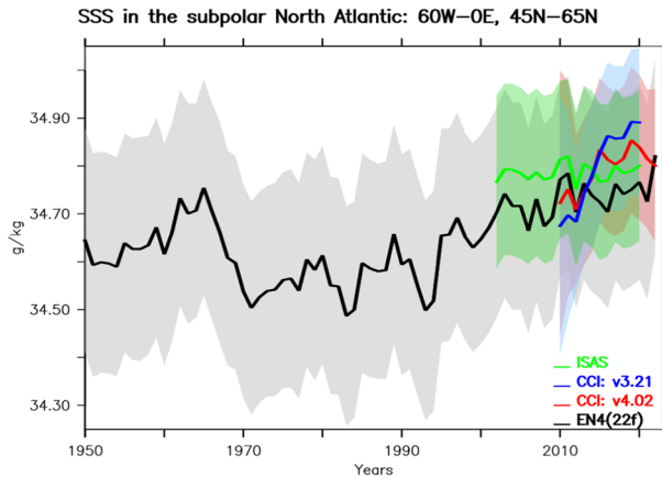
Fig. 2 SSS time series since 1950 averaged the subpolar gyre defined as the box 60–0°W, 45–65°N for different monitoring systems. In black is represented the EN4 product and in green the ISAS products, both of which are mainly based on in situ observation records, notably from ARGO from 2004. In blue and red are recent products from CCI in two different versions (Boutin et al. 2021a, b). The overlap represents an upper estimate of the error for each product. It is estimated as the annual and spatial mean of the uncertainty provided at the gridpoint level. The mask from CCI v4 products using only gridpoints without sea ice has been applied to all products to allow a correct comparison of the data products
