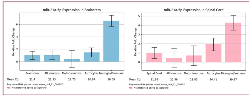
Figure 1. ‘Search by miRNA’ output for miR-21. Expression is consistently enriched in microglial/immune cells within nervous system tissues under physiological conditions ( n = 3\text{--}4 mice; mean \pm SEM). The “Claret” colored frame indicates that miR-21a-5p is broadly conserved among most vertebrate, usually including zebrafish.
