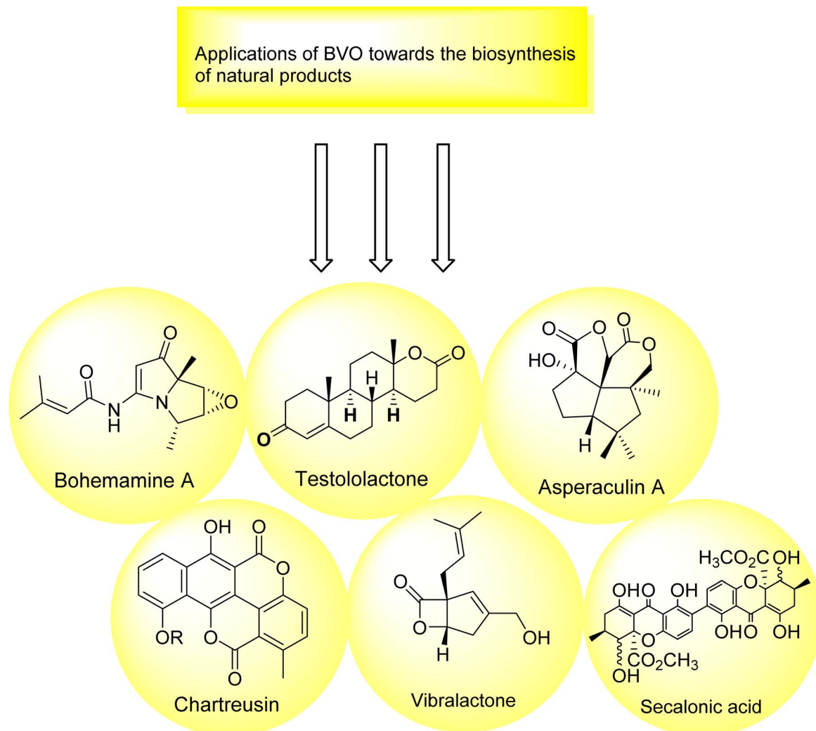
Fig. 7 Pictorial representation of role of BVO in biosynthesis.
