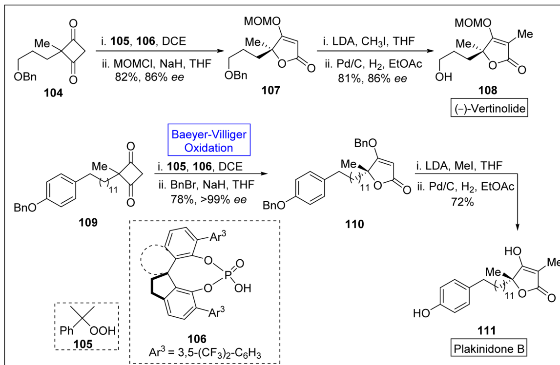
Scheme 13 Synthesis of vertinolide 108 and Plakinidone B 111 via Baeyer–Villiger oxidation.
