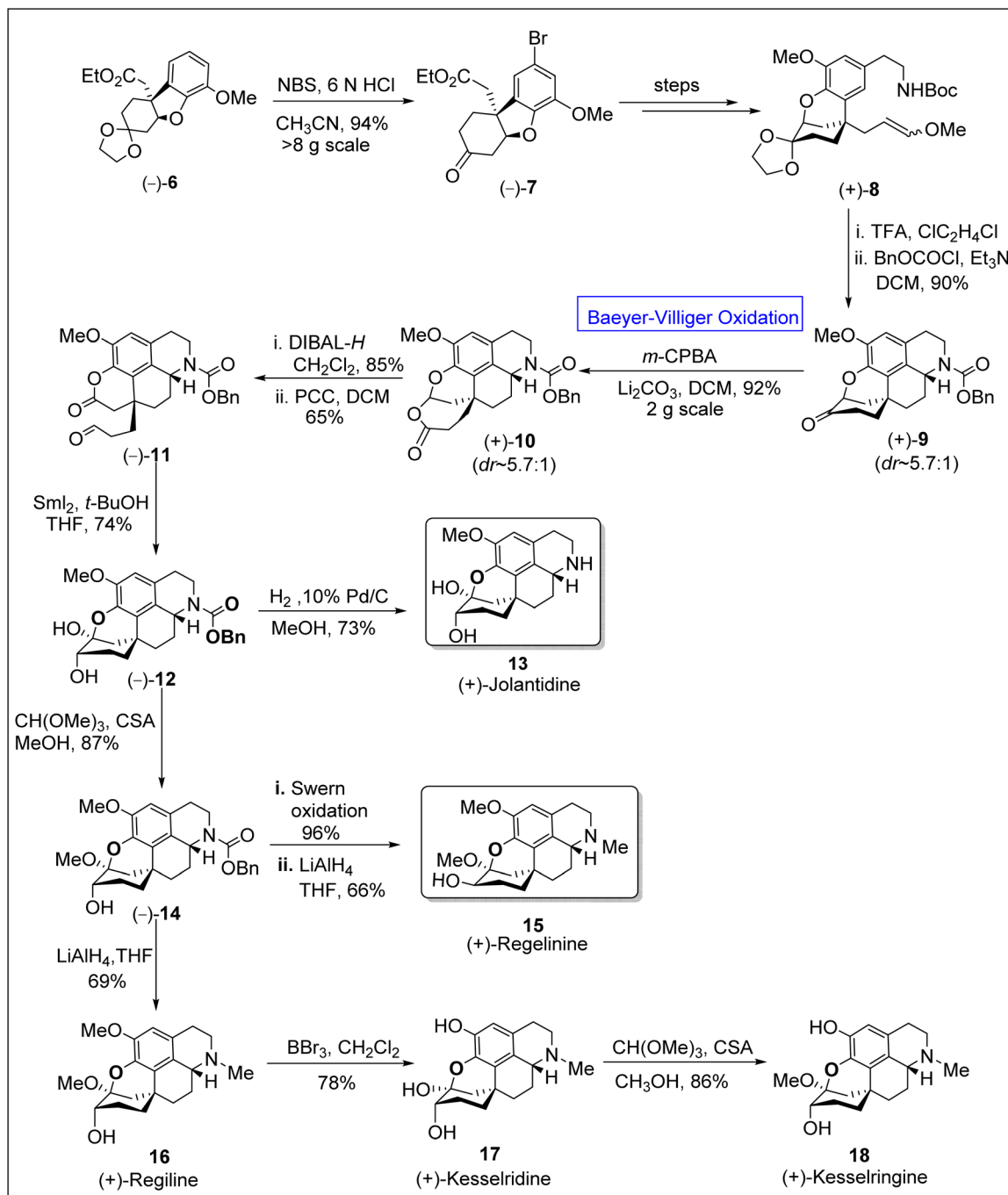
Scheme 2 Synthesis of homoproaporphine alkaloids; joltandine 13 , regelinine 15 , and kesselringine 18 via Baeyer–Villiger oxidation.
