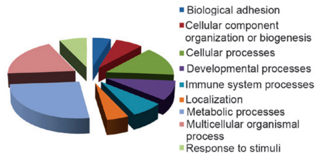
Figure 4. Functional classification of identified proteins in the soleus muscle of rats with SCI. Pie chart demonstrates functional classifications depending on the biological process related to each protein using Protein Analysis Through Evolutionary Relationships.
