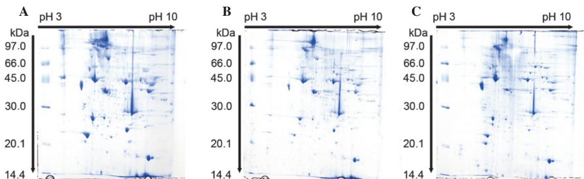
Figure 3. Protein profiles of 2D gel electrophoresis. 2D gels representing proteins from (A) the control group, (B) group 1 (7 days post-SCI) and (C) group 2 (14 days post-SCI). P < 0.05 , n = 3 . SCI, spinal cord injury.
