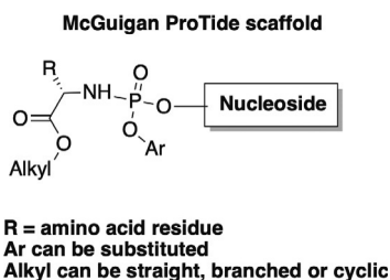
Fig. 8 General structure of the McGuigan ProTide.
