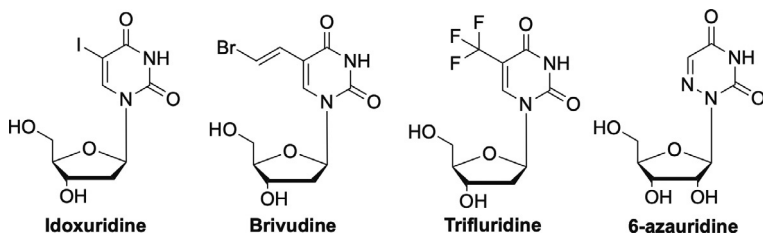
Fig. 1 Early modified nucleoside analogues idoxuridine, brivudine, trifluridine, and 6-azauridine.
