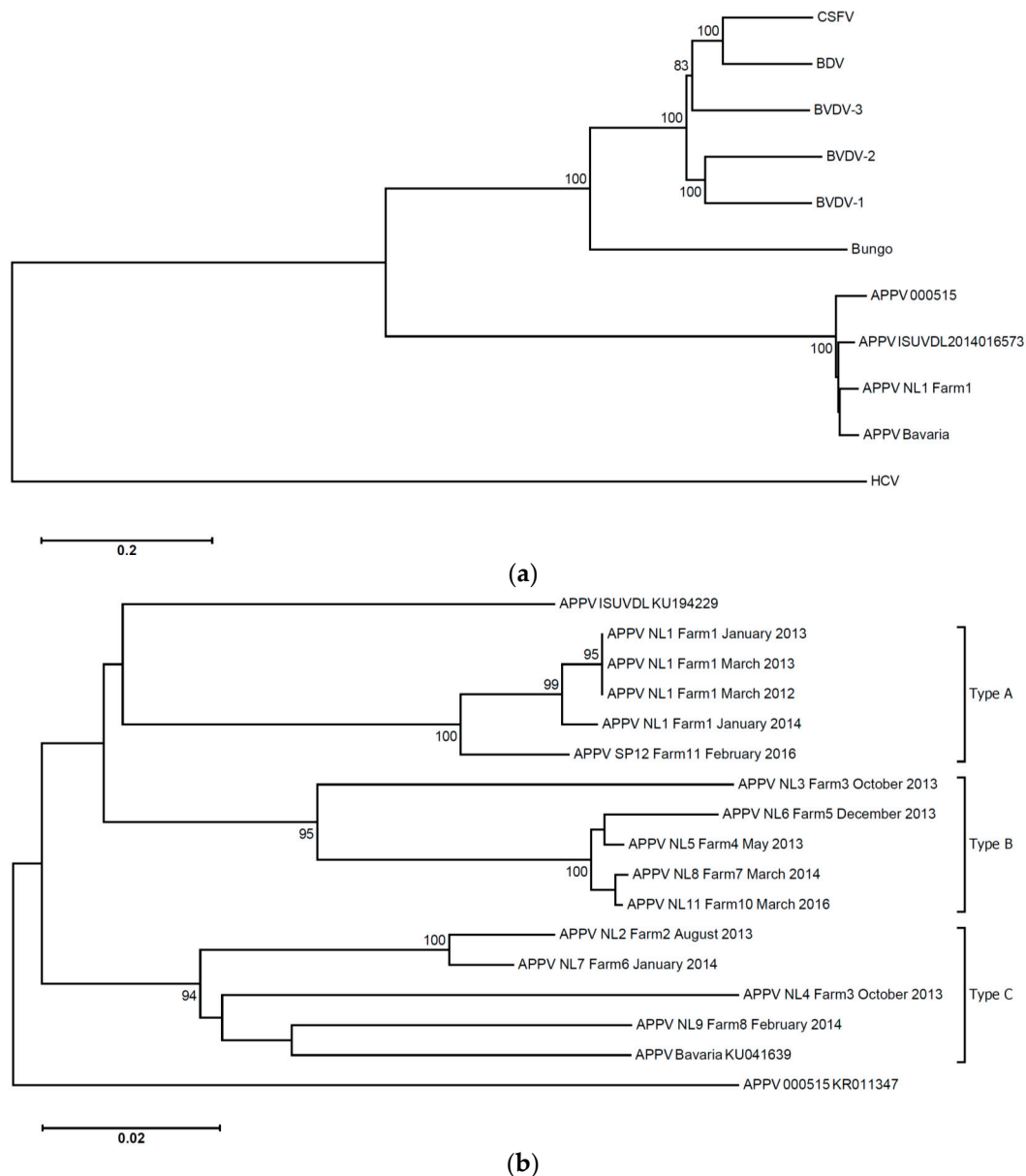
Figure 1. Phylogenetic analysis of the entire coding region (amino acid alignment) of atypical porcine pestivirus (APPV) NL1 Farm1, March 2012, among the known pestiviruses (a) and phylogenetic clustering (nucleotide alignment) into various APPV types (b). The neighbor-joining method with complete deletion within the MEGA-6.06 package was used; bootstrap values above 80 (for 500 replications) are provided at the root of the clusters. The scale bar is a measure of the proportion of divergence. Hepatitis C virus (NC004102.1) is used as the outgroup in (a). BVDV-3: bovine viral diarrhea virus 3 (NC_012812.1); BDV: border disease virus (NC_003679.1); CSFV: classical swine fever virus (NC_002657.1); BVDV-2: bovine viral diarrhea virus genotype 2 (NC_002032.1); BVDV-1: bovine viral diarrhea virus 1 (NC_001461.1); Bungo: Bungowannah porcine pestivirus (NC_023176.1); APPV 000515: isolate 000515 (KR011347.1); APPV of the Iowa State University Veterinary Diagnostic Laboratory (ISUVDL): ISUVDL2014016573 (KU194229); APPV Bavaria: strain S5/9 (KU041639).
