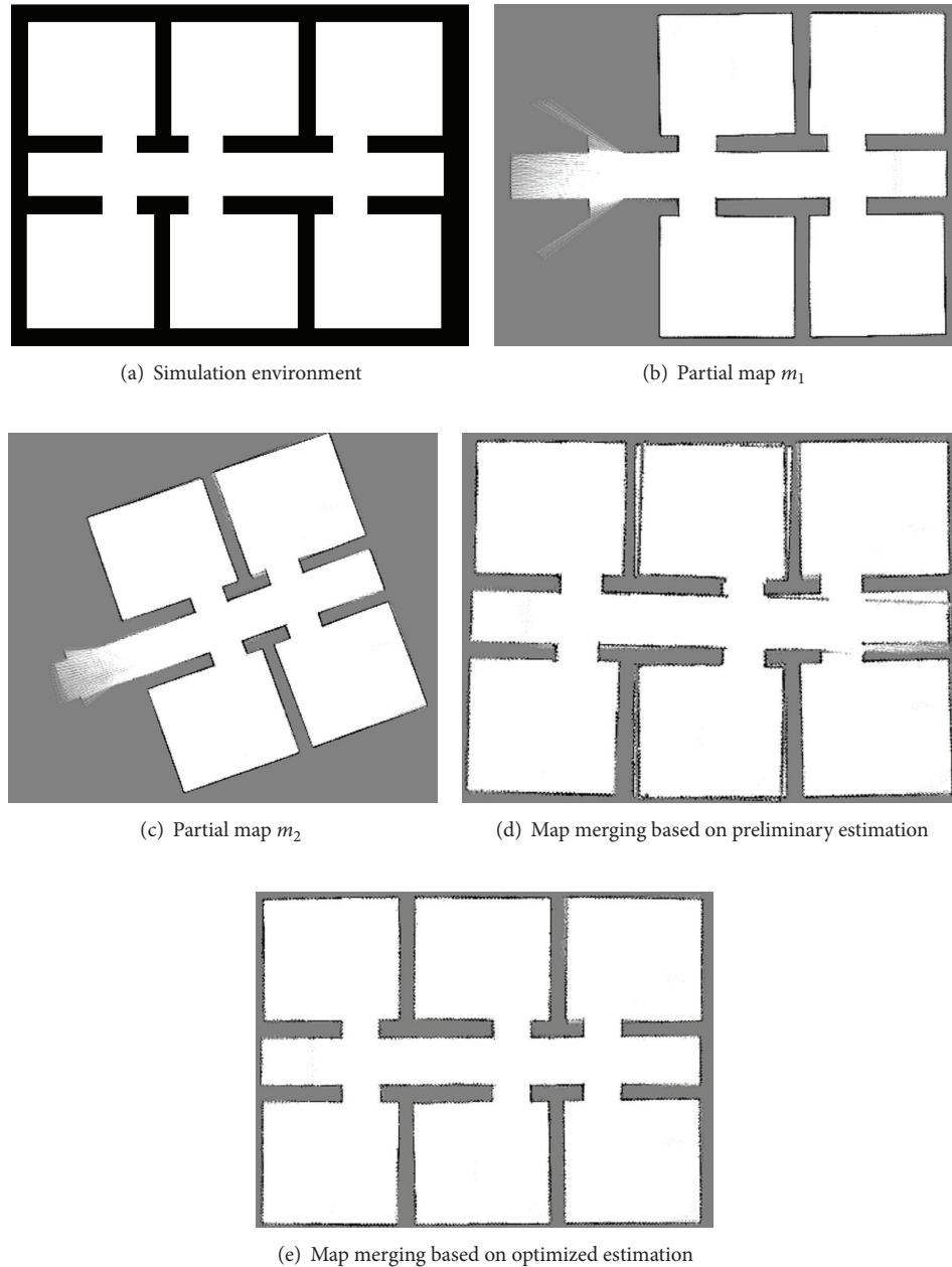
FIGURE 6: Experimental results.
