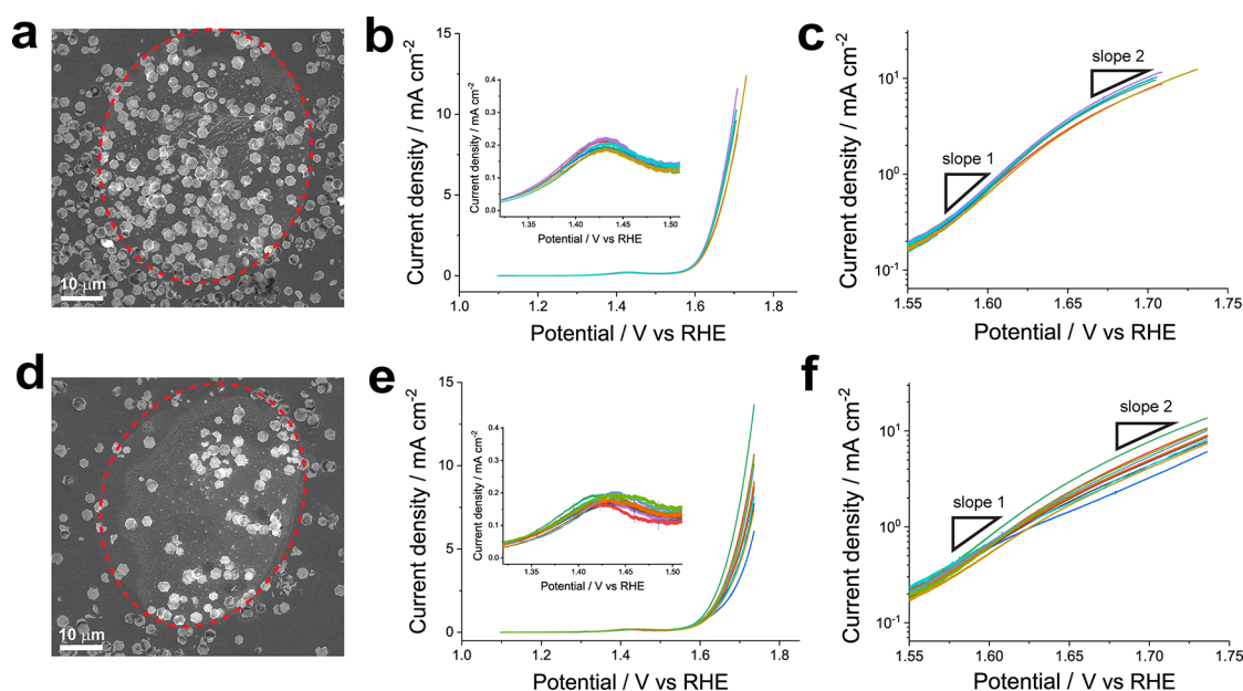
Figure 2. Comparisons of the OER activities of HD and LD \beta -Co(OH) _2 particle ensembles, supported on GC. Representative SEM images for (a) HD and (d) LD particle ensembles with an outline (dotted red), indicating the perimeter of the meniscus cell during SECCM measurements. LSVs ( v = 10 \text{ mV s}^{-1} ) of individual (b) HD ( N = 6 ) and (e) LD ( N = 12 ) particle ensembles and their corresponding (c, f, respectively) Tafel plots. The SECCM experiments were carried out using a single-channel micropipet probe with d_{\text{tip}} = 55 \text{ }\mu\text{m} filled with 0.1 M KOH.
