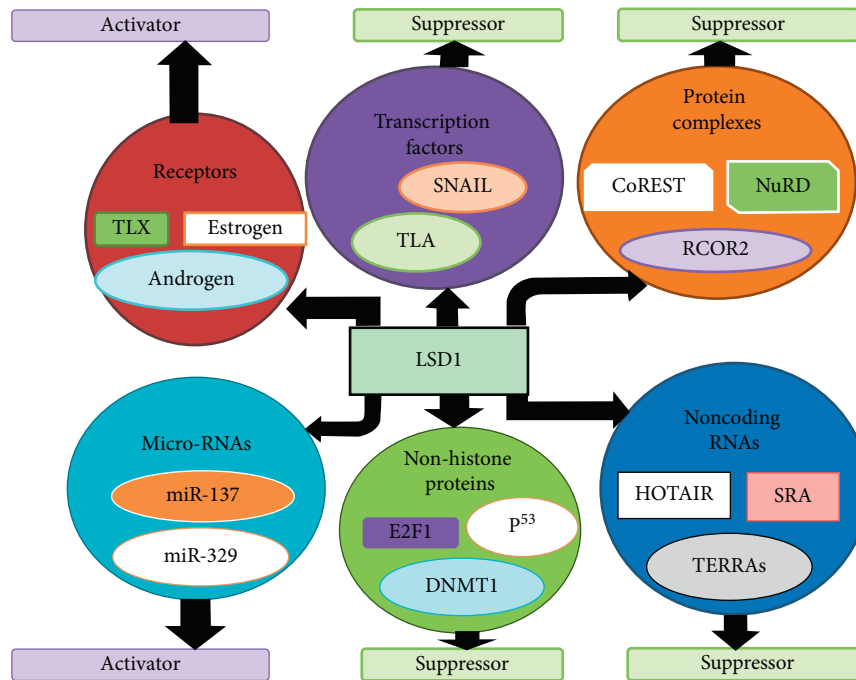
FIGURE 1: LSD1 interacting partners and functional diversity [18]. LSD1 contains several protein complexes (such as “NuRD and RCOR2”), receptors (such as “estrogen and androgen”), noncoding RNAs (such as “HOTAIR and SRA”), microRNAs (such as “miR-137 and miR-329”), non-histone proteins (such as “p53 and E2F1”), and transcription factors (such as “TLA and SNAIL”). The reaction of LSD1 among varied factors permits the varied directive of diverse biological procedures via the suppression and the activation of target gene expression subject on the mode of its interrelating partners; thus, LSD1 is downregulated when there is the reaction of LSD1 with miR-137 and results in cell differentiation by activating the linked genes. When associated with CoREST, it results in downregulation of LSD1 and suppresses target genes.
