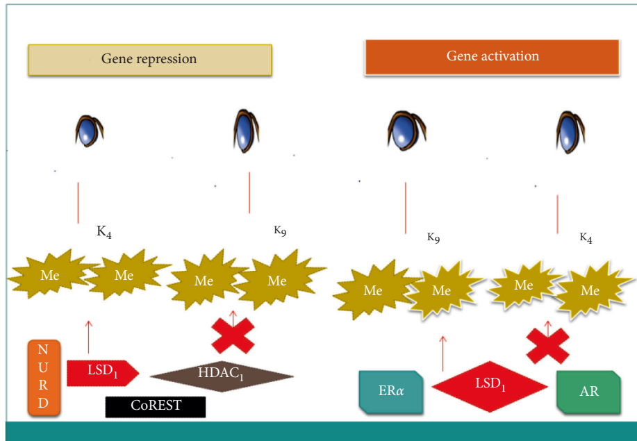
FIGURE 2: Substrate detailed and directive of gene expression by LSD1. For targeted gene expression inhibition, the removal of H3 from H3K4me1/2 was attained by binding LSD1 to CoREST and NuRD complex. The binding of LSD1 to the CoREST and NuRD complex did not speed up the removal of H3 from H3K9me1/2. For targeted gene expression control, the modification of substrate specificity from H3K4me1/2 to H3K9me1/2 was attained by LSD1 binding to androgen and estrogen receptors.
