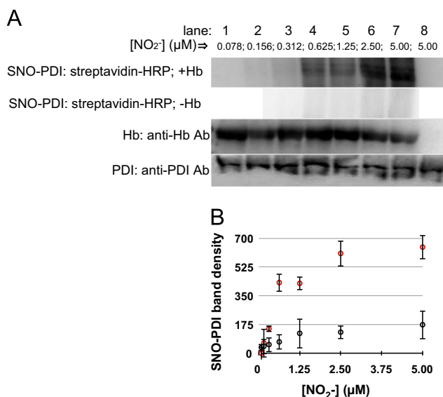
Fig. 3. Hb promotes NO_2^- -dependent nitrosylation of PDI under normoxic conditions (16% O_2 ): (A) These experiments were performed using constant PDI ( 1 \mu M ), Hb ( 0.6 mM) and varying amounts of nitrite ( 78 nM– 5 \mu M ) in PBS-Lanes 1–7. The headspace of the vial contained 16% O_2 . The mixtures were incubated at 37^\circ C for 10 min. Aliquots were then removed and added to cold acetone and prepared for either the SNO-PDI determination by the biotin switch assay-visualized by streptavidin-HRP or detecting Hb or PDI by Western immunoblots utilizing anti-Hb or anti-PDI, respectively as the primary antibodies. Lane 8-only contained PDI ( 1 \mu M ) plus nitrite ( 5 \mu M ) and no Hb. (B) Digitized blot densities (ImageJ) of SNO-PDI as a function of [NO_2^-] in the presence of Hb (red circles) and absence of Hb (black circles). Error bars represent standard deviation ( n=3 ).
