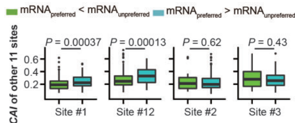
Fig. 6. Codon usage in proximal sequence contexts modulated the relationship between codon optimality and mRNA level. For variant pairs where the only difference is at site #1 of GFP region 2 library, we compared the CAI of other 11 sites between variant pairs showing mRNA_{\text{preferred}} < mRNA_{\text{unpreferred}} and those showing mRNA_{\text{preferred}} > mRNA_{\text{unpreferred}} . The results of three more sites in the library are shown. P values were calculated with Mann–Whitney U test.
