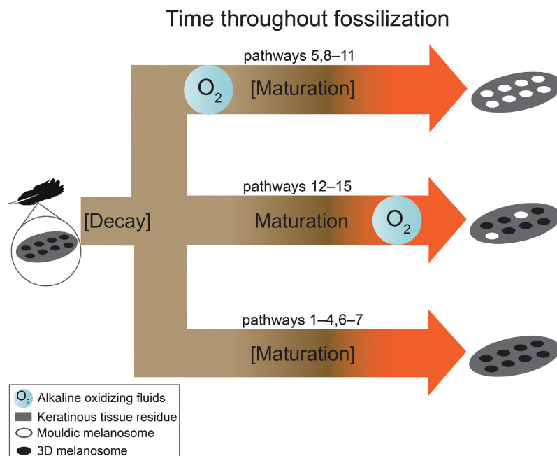
FIG. 7. The impact of various taphonomic conditions on melanosome preservation. Grey ovoid denotes transverse section of feather barbuule. Arrows indicate time. Brackets indicate that a particular taphonomic process is not always present. Pathway 16 is not shown as it involved simultaneous exposure to an oxidant and elevated temperatures, and the presence/absence of melanosomes and moulds could not be confirmed in the degraded residue.
