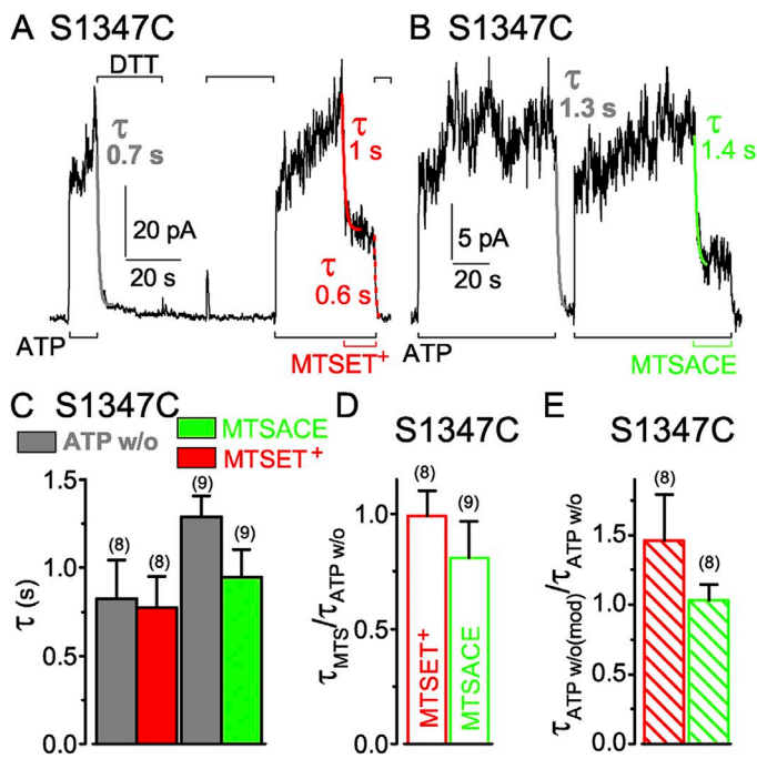
Figure 5. Similarly rapid decay of current in S1347C CFTR channels (containing a single target Cys in the dead composite site) upon ATP washout (w/o) or modification by MTS reagents. (A and B) S1347C CFTR channels were activated by 3 mM ATP (black bars below records) and modified by 1 mM MTSET + or MTSACE (A and B, red and green bars below records, respectively). Colored lines show single-exponential fits to current decay time courses on modification ( \tau_{\text{MTS}} ) by MTSET + (red) or by MTSACE (green), or on ATP removal (gray, \tau_{\text{ATPw/o}} ) before modification, or on ATP removal after MTSET + modification (dotted red, \tau_{\text{ATPw/o(mod)}} ); colored numbers give time constants; the time constants of Ca 2+ -dependent Cl - current decays in these patches were 0.1 s (A) and 0.3 s (B). (C) Average \tau_{\text{ATPw/o}} (gray bars) with corresponding average \tau_{\text{MTS}} from the same patches (left: gray bar, w/o, 0.8 \pm 0.2 s; red bar, \geq 50 \mu\text{M} MTSET + , 0.8 \pm 0.2 s; n = 8 measurements in six patches; right: gray bar, w/o, 1.3 \pm 0.1 s; green bar, \geq 50 \mu\text{M} MTSACE, 0.9 \pm 0.2 s; n = 9 measurements in seven patches). (D) Averages of individual ratios of washout and modification time constants determined for each pair of measurements (from experiments of C; red open bar, \tau_{\text{MTSET}^+}/\tau_{\text{ATPw/o}} , 1.0 \pm 0.1 ; green open bar, \tau_{\text{MTSACE}}/\tau_{\text{ATPw/o}} , 0.8 \pm 0.2 ). (E) Ratio of washout time constants before and after MTSET + and MTSACE modification ( \tau_{\text{ATPw/o(mod)}}/\tau_{\text{ATPw/o}} : red hatched bar, MTSET + , 1.5 \pm 0.3 , n = 8 measurements in six patches; green hatched bar, MTSACE, 1.0 \pm 0.1 ; n = 8 measurements in seven patches);
