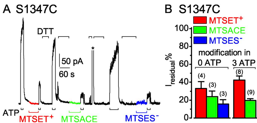
Figure 6. S1347C CFTR channels are readily modified by MTS reagents when closed. (A) Immediately after \sim 60 -s applications of 50 \mu\text{M} MTSET + (red trace and bar), MTSACE (green trace and bar), or MTSES - (blue trace and bar) to closed S1347C channels in the absence of ATP, brief exposures to 3 mM ATP (black bars below record) assessed residual channel activity. Exposures to 20 mM DTT (black bars above record) restored ATP-activated current by releasing adducts after each modification; the asterisk above the record marks brief activation of Ca 2+ -dependent Cl - current to monitor solution exchange speed (time constant = 0.3 s for this patch). (B) Amplitude of residual ATP-dependent
