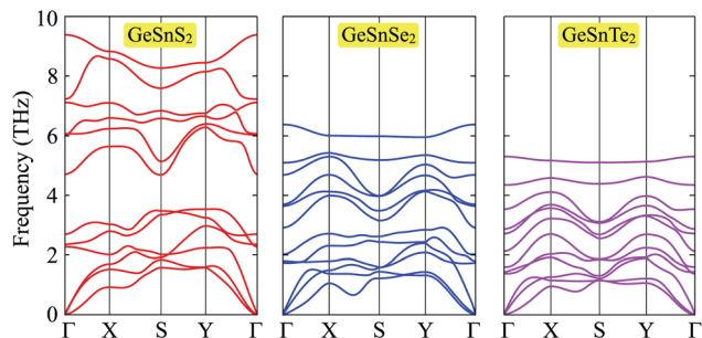
Fig. 2 Phonon spectra of Janus GeSnX 2 single-layers (X = S, Se, Te).
