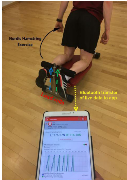
Figure 1 Biodex System 3 eccentric knee flexion apparatus setup (Top). Hamstring Solo Elite pressure feedback device (Bottom).
