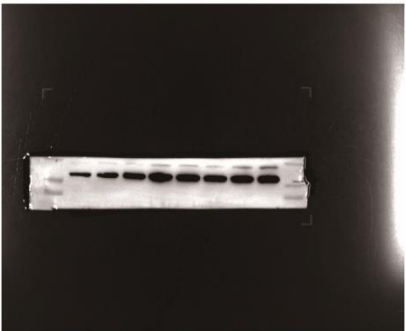
GAPDH
