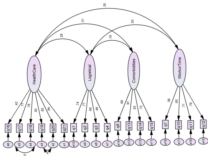
Figure 2 Path diagram for confirmatory factor analysis, displaying the four-factor model, with standardised parameter estimates. Deleted items: 5, 6 and 8 (total items=18/21).
