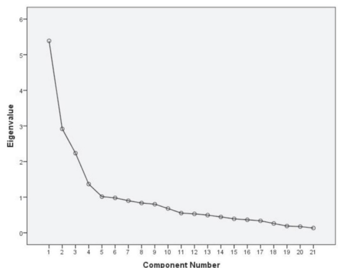
Figure 1 Scree plot from exploratory factor analysis.
