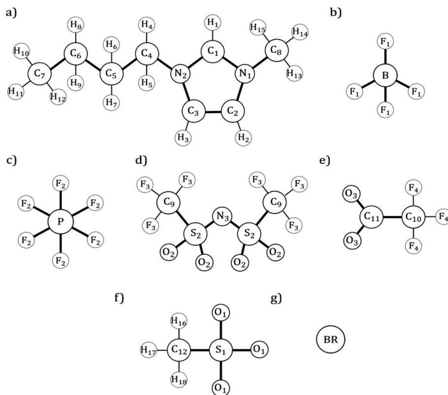
Fig. 1 Schematic representation for all ILs studied (a) 1-butyl-3-methylimidazolium cation [C_4mim]^+ (b) tetrafluoroborate anion [BF_4]^- (c) hexafluorophosphate anion [PF_6]^- (d) bis(trifluoromethylsulfonyl)imide anion [NTf_2]^- (e) trifluoroacetate anion [CF_3COO]^- (f) mesylate anion [OMs]^- (g) bromide anion [Br]^- .
