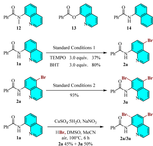
Scheme 3 Mechanistic studies.
