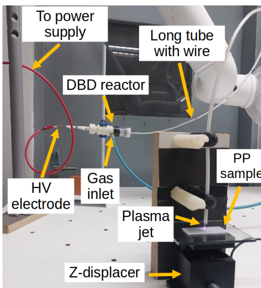
(c) Photo of the plasma device
