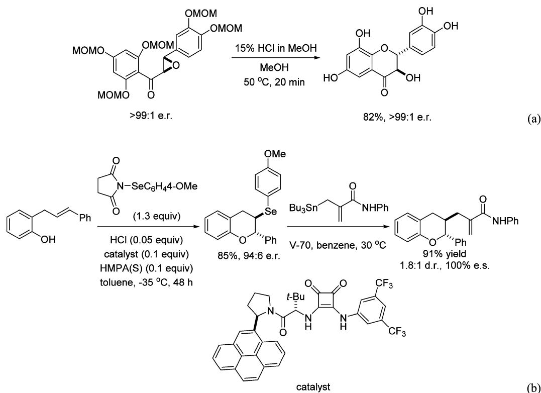
Scheme 3. Synthesis of 2,3-Disubstituted Chromans
