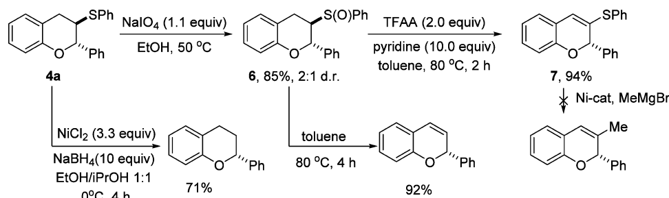
Scheme 5. Manipulations of 3-Phenylthiochroman
