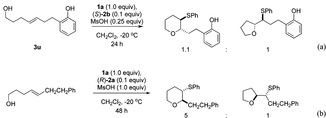
Scheme 7. Constitutional Site Selectivity for 4-Pentenols
