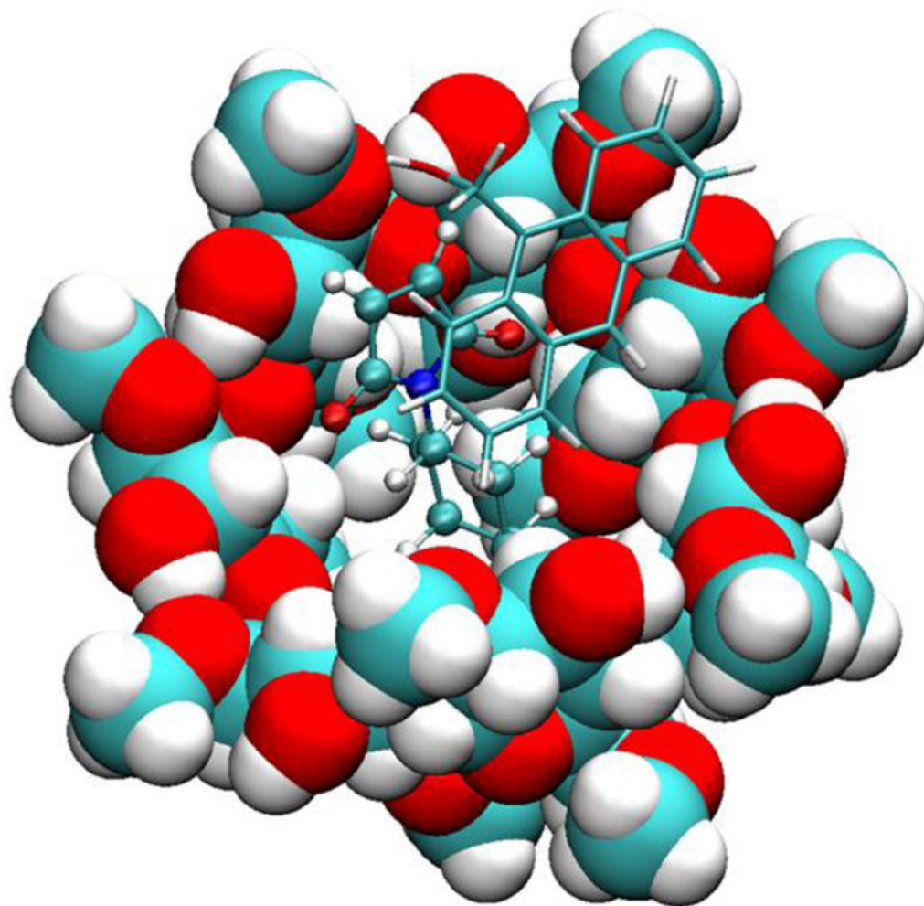
Figure 4. Binding mode of compound 1 with 2a and dimethyl-β-CD. Compound 1 is rendered in licorice, 2a in CPK, and dimethyl-β-CD in VDW.
