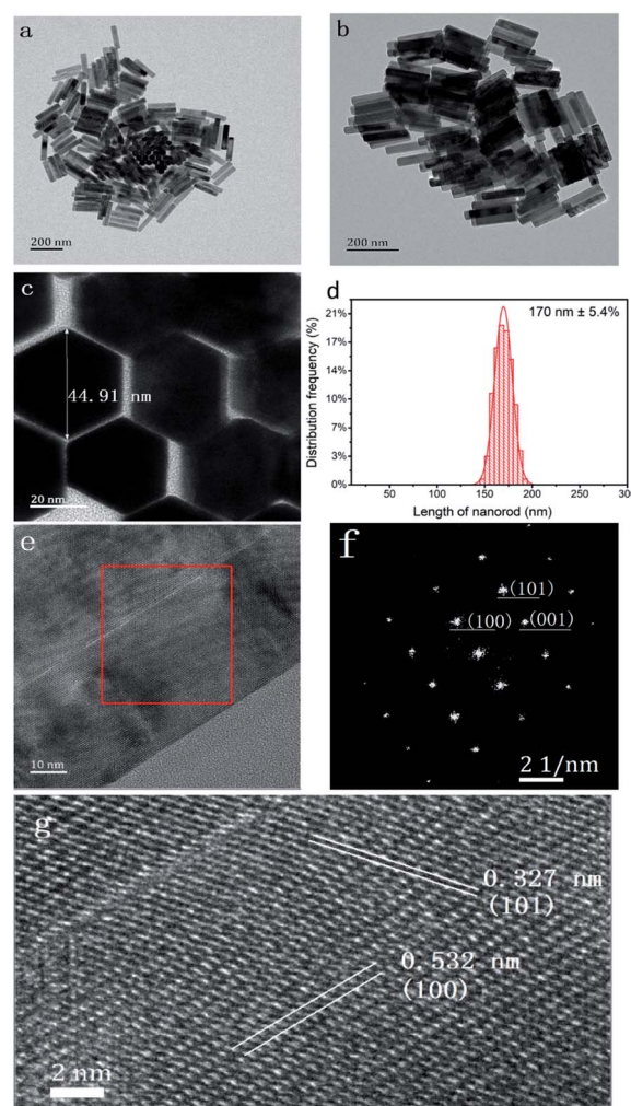
Fig. 1 (a and b) TEM images of \text{NaCeF}_4:20 at% Tb NCs. (c) HRTEM image of the NCs. (d) Distribution frequency of the lengths of the NCs. (e) HRTEM image of the NCs. (f) Fourier transform image of the square area in (e). (g) Zoom in of the square area in (e) with the labelled interplanar spacing.
