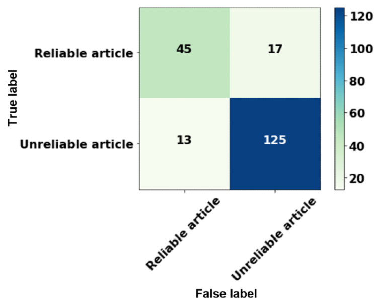
Figure 5. Confusion matrix for ReCOVery validation subset on trained new ensemble model with BiGRU and XGBoost. BiGRU: bidirectional gated recurrent unit; XGBoost: extreme gradient boosting.
