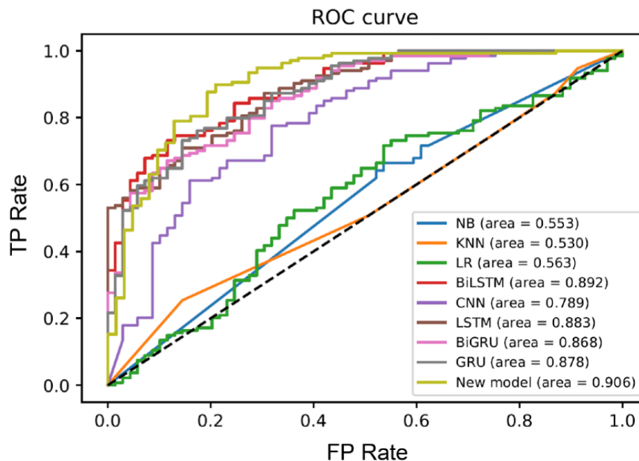
Figure 4. Receiver operating characteristic (ROC) curve and AUC scores with the corresponding color for both traditional ML models (KNN, LR, NB) and deep learning models (BiLSTM, CNN, LSTM, BiGRU, GRU, new model). AUC: area under the curve; BiGRU: bidirectional gated recurrent unit; BiLSTM: bidirectional long short-term memory; CNN: convolutional neural network; FP: false positive; GRU: gated recurrent unit; KNN: K-nearest neighbor; LR: logistic regression; LSTM: long short-term memory; ML: machine learning; NB: naive Bayes; TP: true positive.
