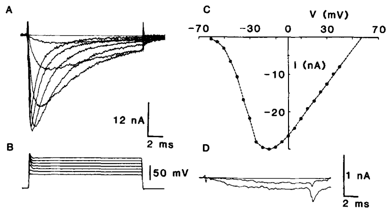
FIGURE 5. Inward currents recorded in voltage-clamped cells with an electrode containing CsF. ( A ) Sodium currents generated by potential steps from a holding potential of -100 \text{ mV} to potentials between -50 and +10 \text{ mV} ( B : 10\text{-mV} increments). ( C ) Current-voltage curve from the same cell as in A . The extrapolated null potential was +58 \text{ mV} . ( D ) Currents recorded in the presence of 1 \mu\text{M} TTX in response to voltage steps to -40 and -50 \text{ mV} from a holding potential of -100 \text{ mV} . These were the largest inward currents seen in the presence of TTX.
