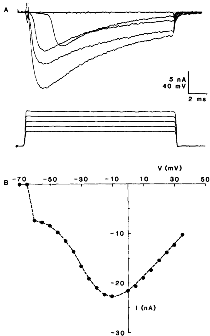
FIGURE 4. "Breakthrough" sodium currents (upper traces) generated by voltage steps (lower traces) to between -60 and -30 mV from a holding potential of -100 mV. (B) The peak current-voltage curve for the currents shown in A contains an obvious discontinuity at -60 mV.
