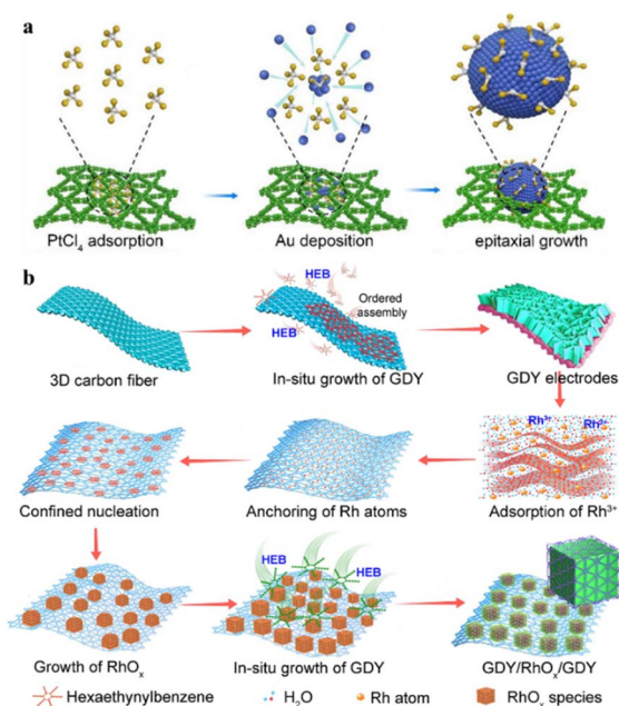
Fig. 12 (a) Synthesis of \text{PtCl}_2\text{Au}(111)/\text{GDY} . Adapted from ref. 66. Copyright 2022, American Chemical Society. (b) Synthesis schematic of the \text{GDY}/\text{RhO}_x/\text{GDY} electrodes. Adapted from ref. 76. Copyright 2022, National Academy of Science.
