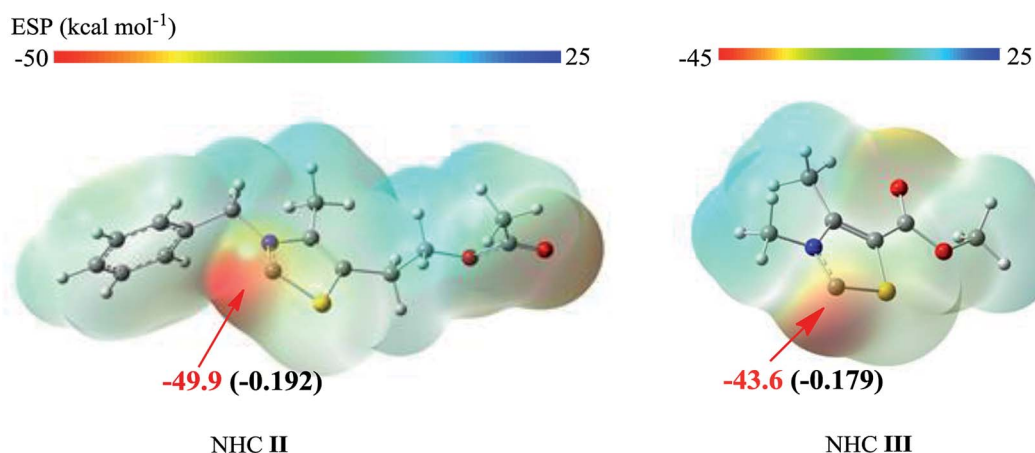
Fig. 5 ESP on the van der Waals surface of NHC II and NHC III. Surface local minima and maxima of ESP are represented as red and blue spheres, respectively. Only the global minima are labeled. The values in parentheses are calculated Hirshfeld charges.
