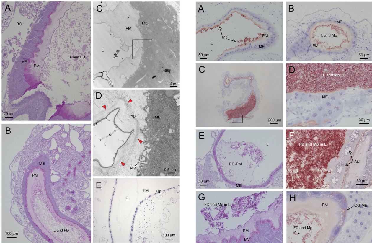
Fig. 2. Observations of non-infected control larvae. A and B, PAS staining of larva nos. 3 and 5 at 72 hpi, respectively. The surfaces of PM show strong positivity for PAS, and the interface between the PM and the lumen is clear. C, Transmission electron micrographs of larva no. 9 at 72 hpi. D, High magnification of boxed area in panel C. The PMs do not have constant thickness, having rough surfaces and low electron density with a granular appearance and partially showing some layers inside (red arrowheads in panel D). E, IHC stain of larva no. 10 at 84 hpi with anti- M. plutonius serum. No positive signal is observed. PM, peritrophic matrix; ME, midgut epithelial cell; L, lumen; FD, food in the midgut; BC, body cavity; MV, microvilli.
