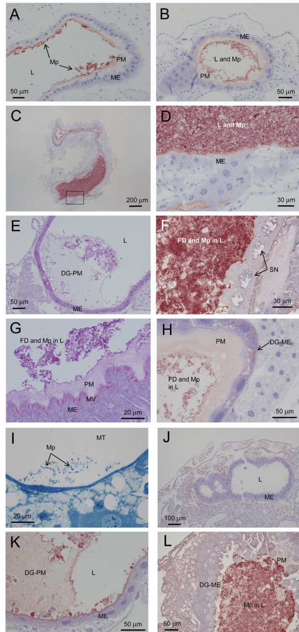
Fig. 3. Light microscopic observations of strain DAT561-infected larvae. A, IHC stain of larva no. 31 at 72 hpi. DAT561 cells are localized in the midgut lumen and attach to the surface of the PM. B, IHC stain of larva no. 32 at 72 hpi. DAT561 mass extended towards the lumen. C, IHC stain of larva no. 33 at 72 hpi. D, High magnification of boxed area in panel C. The midgut lumen is filled with DAT561 cells. E, PAS stain of larva no. 48 at 108 hpi. The PM is considered to have degenerated. F IHC stain of DAT561-infected larva no. 55 at 120 hpi. Swollen nuclei are observed in the midgut epithelial cells, and bacteria directly attach to the midgut epithelial cells. G, PAS stain of DAT561-infected larva no. 31 at 72 hpi. Intact microvilli are observed on the apical surfaces of the epithelial cells. H, IHC stain of DAT561-infected larva no. 49 at 108 hpi. The midgut epithelial cells have many vacuoles. I, MB stain of larva no. 44 at 84 hpi. A few bacteria exist in the Malpighian tubules. J, IHC stain of larva no. 47 at 108 hpi. Positive signals are detected all over the larval body. K, IHC stain of larva no. 48 at 108 hpi. Luminal side of the epithelial cells is strongly stained with the anti- M. plutonius serum. Degenerated PM also shows positive reaction. L, IHC stain of larva no. 53 at 120 hpi. In addition to intact bacterial cells, IHC-positive bacterial antigens are detected throughout the larval body. FD, food in the midgut; Mp, M. plutonius ; L, lumen; PM, peritrophic matrix; DG-PM, degenerated PM; MV, microvilli; ME, midgut epithelial cell; DG-ME, degenerated ME; SN, swollen nuclei; MT, the Malpighian tubule.
