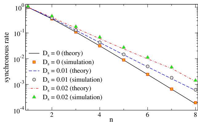
Fig. 3 Mean of the synchronous output (“synchronous firing rate”) vs number of spike trains for different amplitudes of the signal as indicated and a cut-off frequency of f_c = 10
