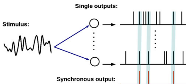
Fig. 1 Model of n noisy neurons, which are driven by a common broadband noise. Given the spikes generated by the single neurons (upper time traces), the synchronous output of the population (lower time trace) shows spikes only if all of the neurons fire a spike in close temporal neighborhood. The main question in this paper is, how much information the synchronous output carries about the common stimulus in different frequency bands
