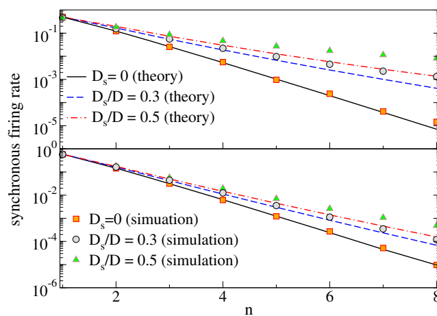
Fig. 6 The mean synchronous output (‘synchronous firing rate’) of LIF neurons as a function of the population size n for different signal intensities as indicated. Parameters: \mu = 0.8 , D = 0.2 (upper panel); \mu = 1.2 , D = 0.01 (lower panel)
