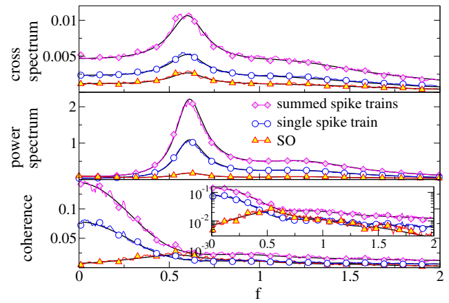
Fig. 9 Spectral measures of the single and summed spike trains, and the SO for LIF neurons in the suprathreshold (deterministic) firing regime. Parameters: n = 2 , \mu = 1.2 , D = 0.01 and D_s = 0.001
