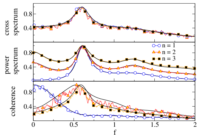
Fig. 10 Spectral measures of the SO for LIF neurons in the suprathreshold (deterministic) firing regime for different numbers of neurons as indicated. All curves are rescaled to their respective maximum. Note that while cross-spectra are very similar, the width of the spectral peak in the power spectra depends on n and because of the increasing width, the coherence for n > 1 shows a maximum vs frequency. Parameters: \mu = 1.2 , D = 0.01 and D_s = 0.001
