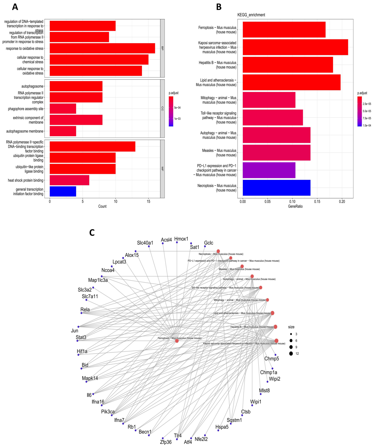
Figure 3 Enrichment analysis of 82 FRDEGs. (A) GO enrichment analysis of 82 FRDEGs. (B and C) KEGG enrichment analysis of 82 FRDEGs.
