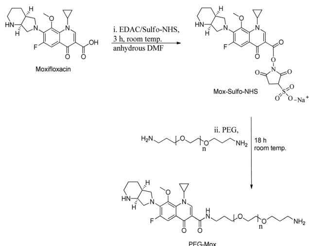
Fig. 1 Schematic of the synthesis of the PEG–Mox conjugate using carbodiimide chemistry.
