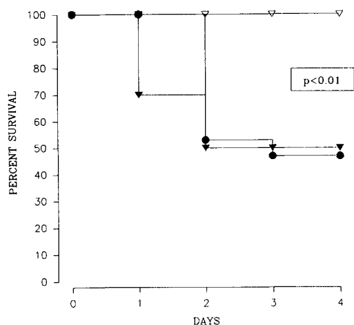
Figure 3. Lethality after injection of 500 \mu g LPS in three groups of BALB/c mice: (●) mice with no pretreatment ( n = 15 ); (▽) mice pretreated intraperitoneally with 1,000 U IL-10 ( n = 15 ); (▼) mice pretreated intraperitoneally with supernatant from mock-transfected CHO-K1 cells ( n = 10 ). Two-tailed p value has been determined with the Fisher's exact test.
