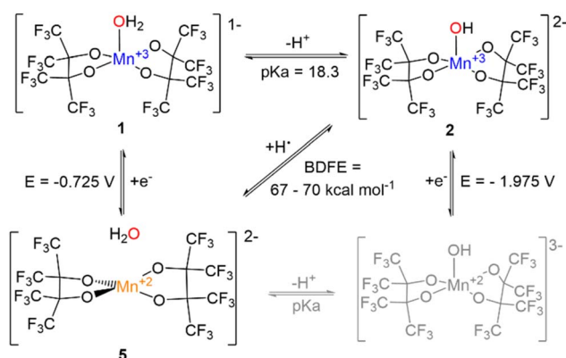
Scheme 6 Bordwell scheme depicting the proton, electron, and hydrogen atom transfer events and their respective thermodynamic parameter for the [Mn(OH x )(pin F ) 2 ] 2- system. Gray indicates a proposed, not isolated species.
